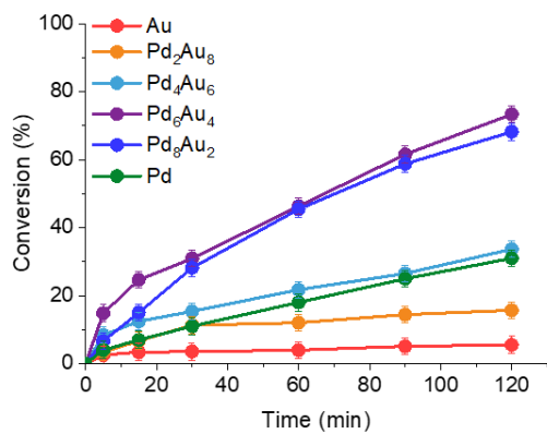
Figure 6. Conversion as a function of reaction time of the different 1%PdxAu@HHT catalysts for the liquid phase dehydrogenation reaction of FA under mild condition.
