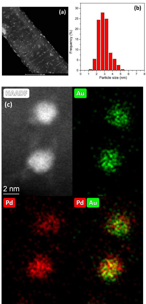
Figure 1. a) STEM-HAADF image of 1%Pd 0 Au 0 @HHT catalyst, b) particle size distribution and c) STEM-EDS maps of single nanoparticles.
