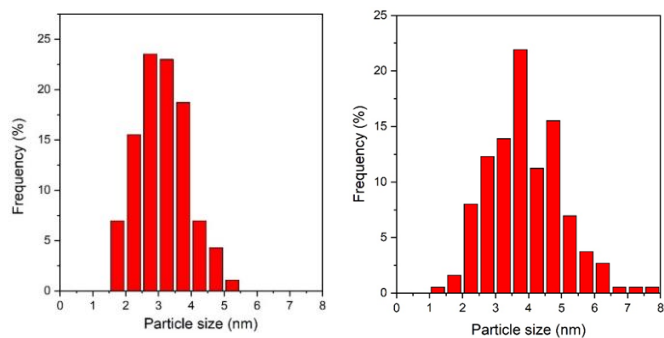
Figure 8. Average particle size distribution of a) used 1%Pd 6 Au 4 @HHT and b) used 1%Pd 6 Au 2 @HHT
