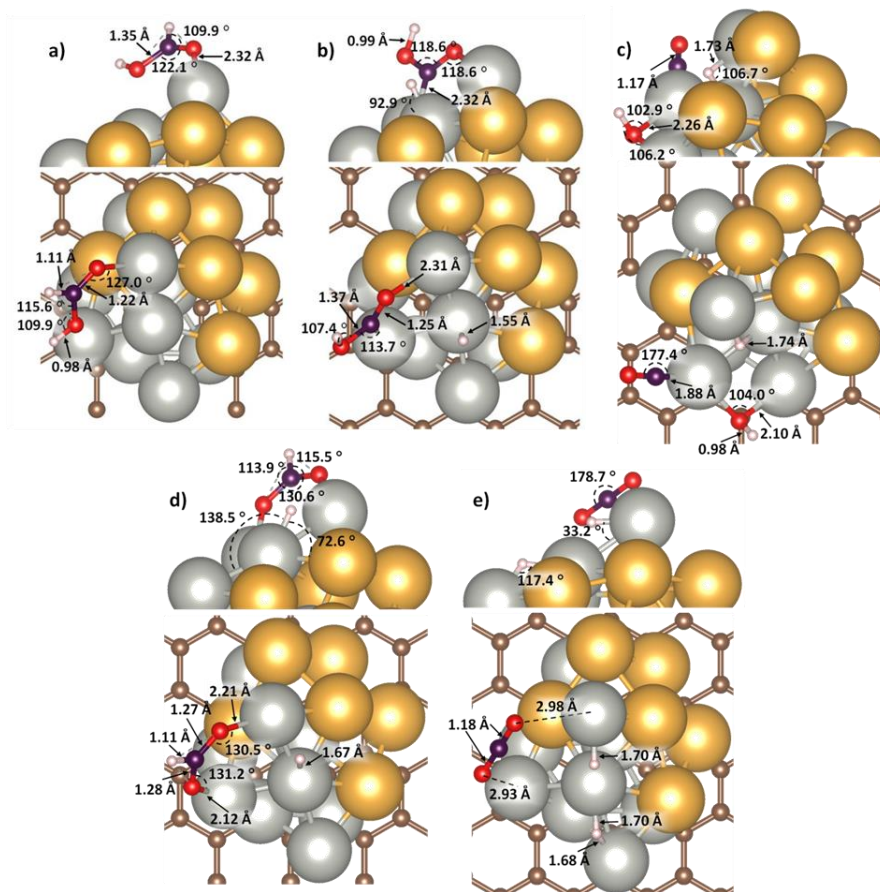
Figure 12. Top and side views of the optimized elementary steps on \text{Pd}_5\text{Au}_6 cluster; (a) FA adsorbed on the cluster, (b) COOH and H adsorbed after the dissociation of the C-H bond, (c) CO, H and OH adsorbed after the dissociation of the C-OH bond, (d) HCOO and H adsorbed after the dissociation of the O-H bond and (e) H and H adsorbed on the cluster after the dissociation of C-H bond. \text{CO}_2 is more stable in gas phase than adsorbed. Insets show distances and angles of interest. Carbon atoms are represented in brown, gold atoms in gold, palladium in silver, oxygen in red, hydrogen in white and the carbon atoms of formic acid in purple.
