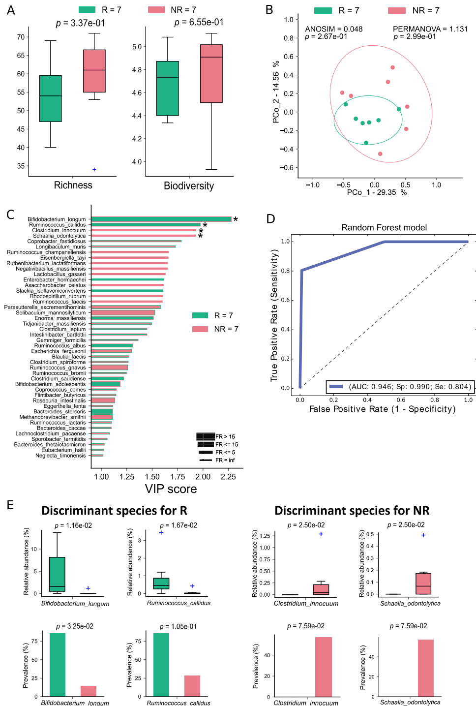
Fig. 2. Microbiota compositional shifts in responders and non-responders. Alpha- (A) and \beta -diversity (B) of responders (R, green, n = 7 ) and non-responders patients (NR, red, n = 7 ). (C) Variable Importance Plot (VIP). It shows: (i) discriminant species after Partial Least Square Discriminant Analysis (PLS-DA) in descending order of VIP score (bar length); (ii) the highest relative abundance depending on the cohort (central bar colour) and the lowest one (edge bar colour); (iii) fold ratio (FR) of the highest versus the lowest relative abundance (bar thickness), and (iv) significant difference after Mann–Whitney U test (non-false discovery rate [non-FDR], *p \leq 0.05 ). Absent borders indicate mean relative abundance of zero in the compared cohort. (D) Receiver Operating Characteristic (ROC) curve with fivefold cross-validation following a Random Forest model on the four species (retrieved by the VIP plot). Area Under Curve (AUC), sensitivity (Se) and specificity (Sp) are reported. (E) Pairwise analysis of the selected four species depicts significant differences in terms of relative abundance (box plots) and prevalence (bar plots). In each sub-graph are reported the p -value (from Mann–Whitney U test) among R and NR. Blue crosses are outliers.
