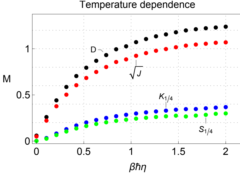
Figure 2: Plot of the non-Markovianity measure for the spin-boson dephasing model in its dependence on the inverse temperature, for the different quantifiers D , \sqrt{J} , K_{1/4} and S_{1/4} .
