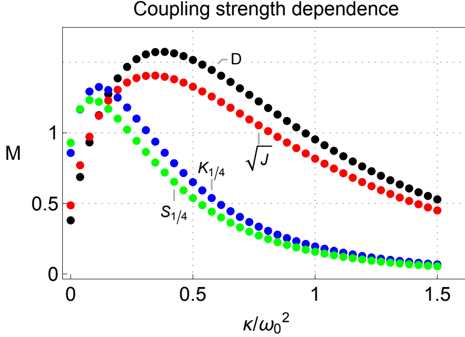
Figure 3: The same as in Fig. 2, but considering the coupling strength dependence of the non-Markovianity measure.
