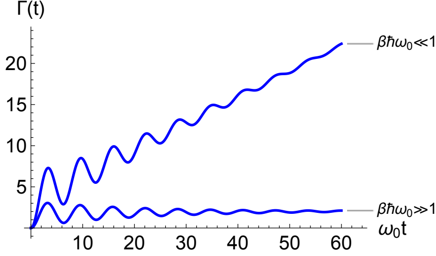
Figure 1: Behavior at high and low temperature of the decoherence function \Gamma(t) given by Eq. (46), obtained considering the spectral density of Eq. (44) and a thermal environmental state with inverse temperature \beta .
