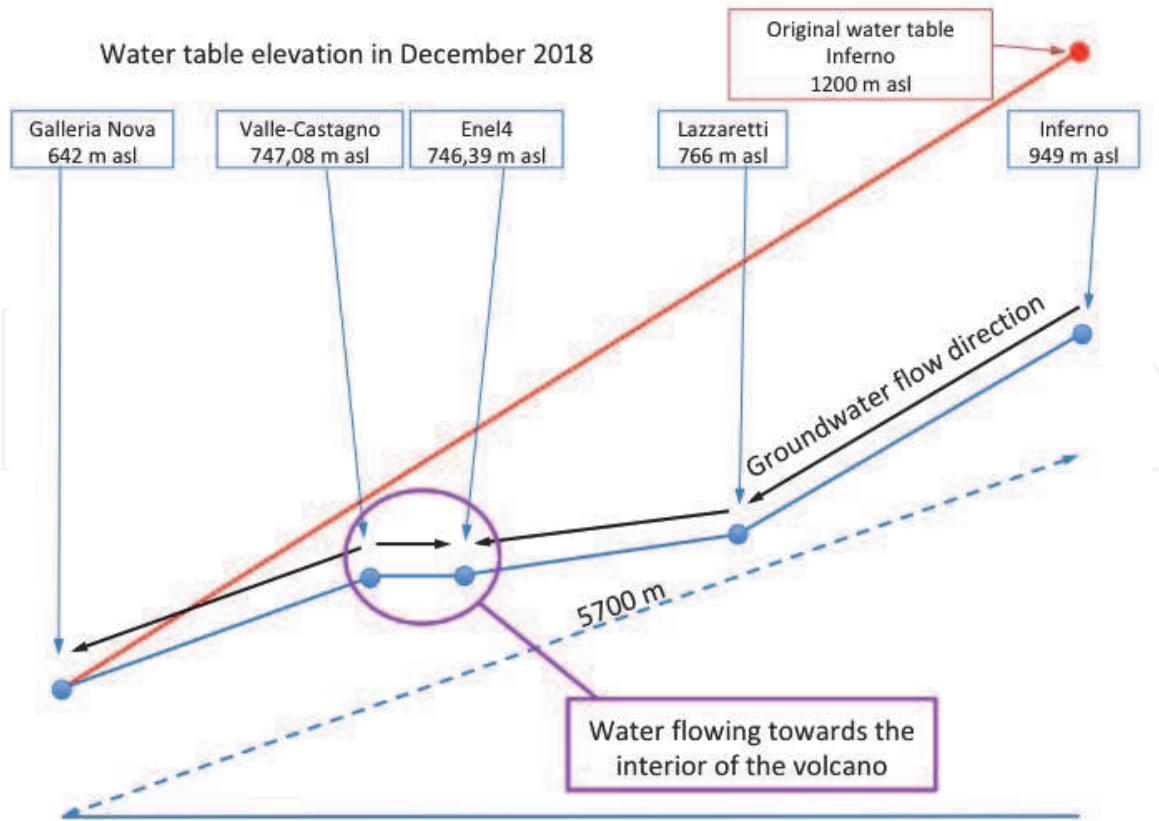
Figure 7. Sketch of water table levels measured in December 2018. Red line is the approximate original water table from Figure 3a. The elevation of the water table inferred by projected piezometer data from “ENEL Valle” and “ENEL Castagno” is the linear interpolation between their two elevations. Note: (1) the reduction in the water table and (2) the flow of water that is from the Valle-Castagno piezometers (located at lower topographic elevations) toward the ENEL4 piezometer (located at a higher topographic elevation) shows an inversion in the original direction of water flow in the aquifer. Data from Regione Toscana—Centro Funzionale Monitoraggio Idrologico-Idraulico.
