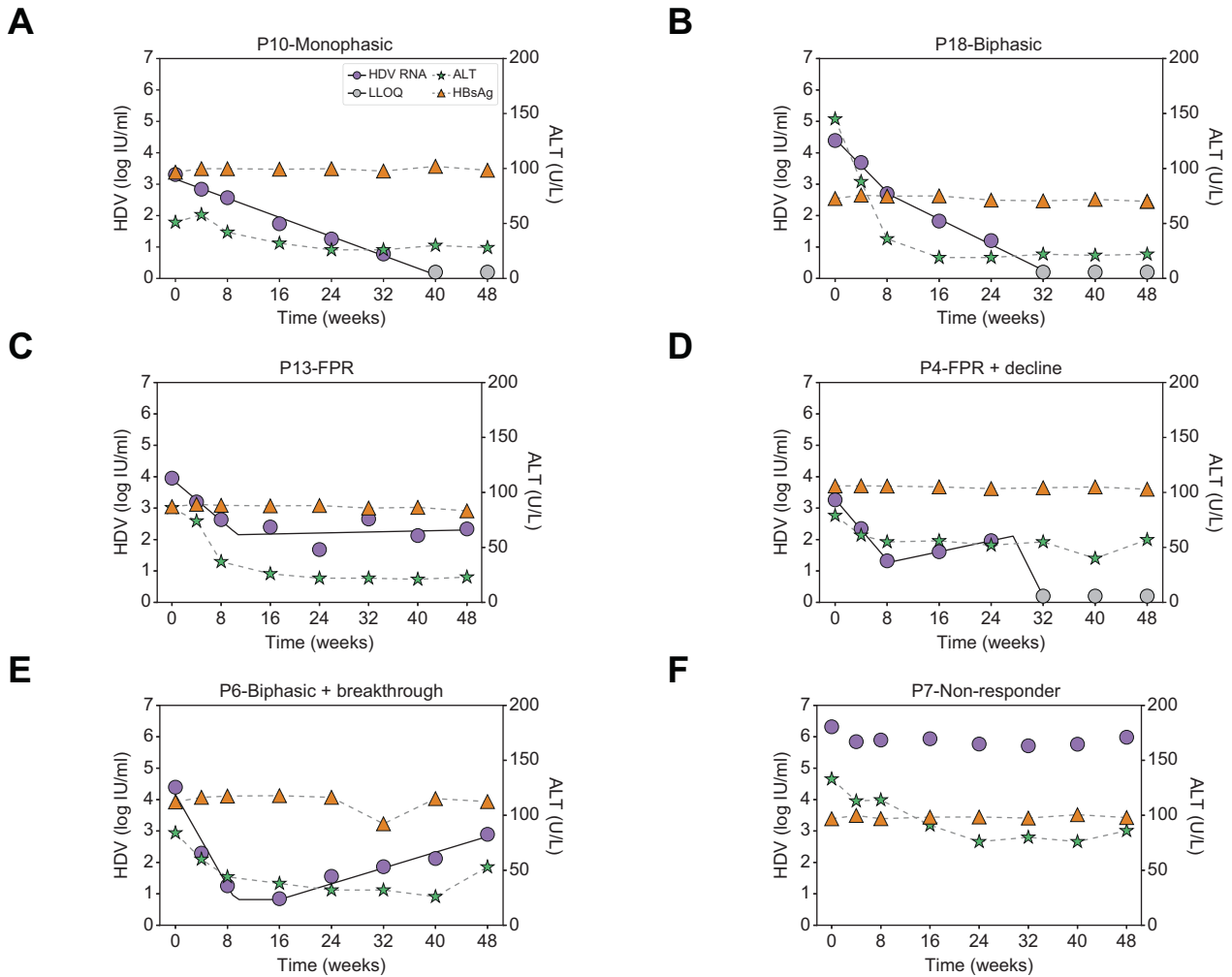
Fig. 2. HDV kinetic patterns under BLV monotherapy in patients with compensated cirrhosis and clinically significant portal hypertension. (A) Monophasic, i.e. a single phase of viral decline ( n = 2 ), (B) biphasic, viral decline consisting of a first phase decline that was 2-fold faster than the second phase decline ( n = 8 ), (C) FPR, defined as a first phase viral decline followed by a plateau that was not significantly ( p > 0.05 ) different from slope=0 ( n = 3 ), (D) FPR followed by decline ( n = 1 ), (E) Biphasic followed by breakthrough ( n = 2 ), and (F) non-responder, defined as having < -1.0 log IU/ml decline from baseline ( n = 2 ). Solid lines for HDV reflect modelling using piecewise linear regression and dashed lines between ALT markers are shown only to highlight the trajectory. ALT, alanine aminotransferase; BLV, bulevirtide; FPR, flat-partial response; HDV, hepatitis D virus.
