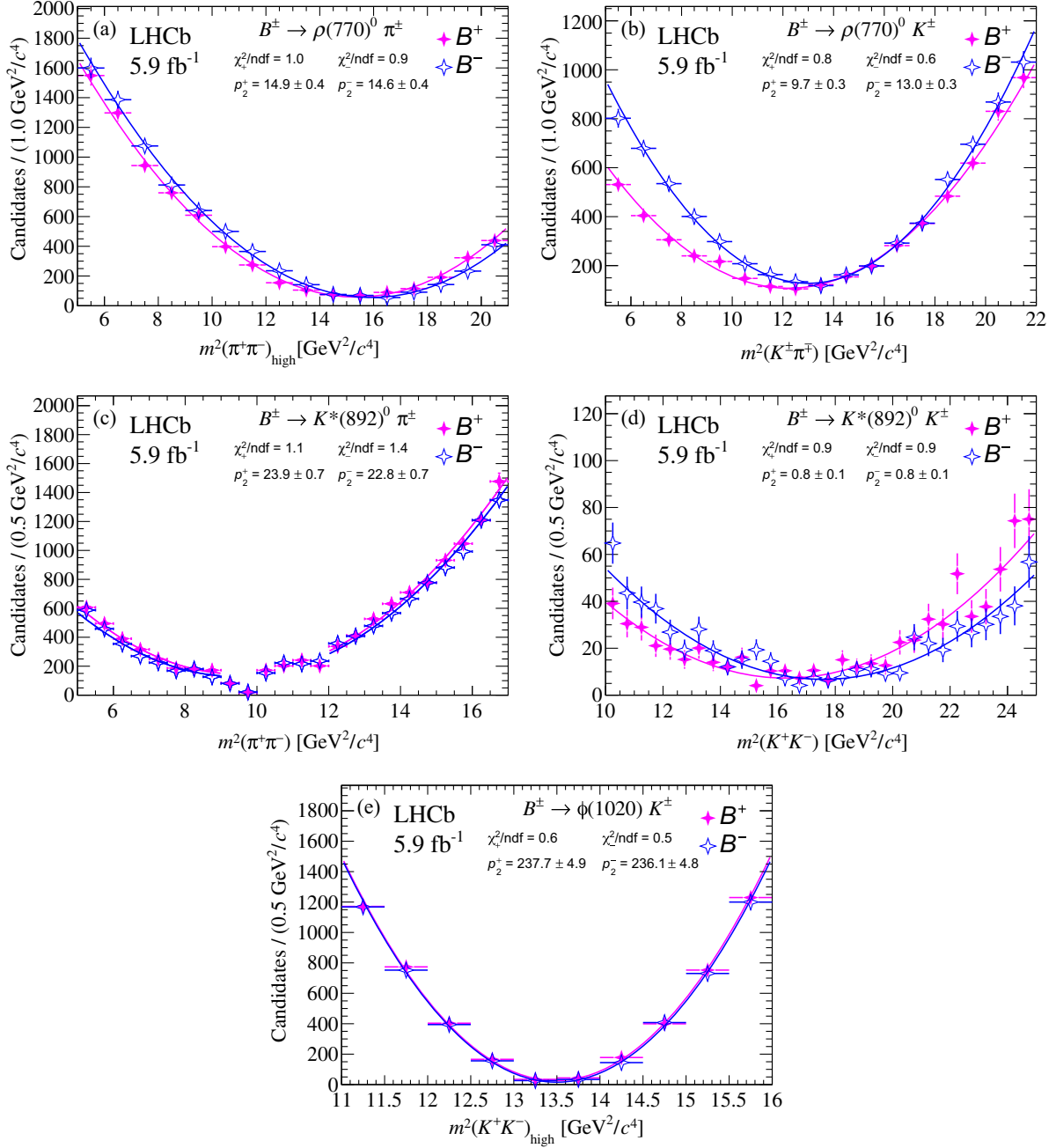
FIG. 1. Distribution of s_{\perp} for B^+ and B^- candidates and the corresponding quadratic fits for (a) \rho(770)^0 in B^{\pm} \rightarrow \pi^{\pm}\pi^+\pi^- , (b) \rho(770)^0 in B^{\pm} \rightarrow K^{\pm}\pi^+\pi^- , (c) K^*(892)^0 in B^{\pm} \rightarrow K^{\pm}\pi^+\pi^- , (d) K^*(892)^0 in B^{\pm} \rightarrow \pi^{\pm}K^+K^- , and (e) \phi(1020) in B^{\pm} \rightarrow K^{\pm}K^+K^- . In the symmetric channels, the phase space distribution and its projections are presented with the two axes being the squares of the low-mass m_{\text{low}} and high-mass m_{\text{high}} combinations of the opposite-sign particle pairs, for visualization purposes.
