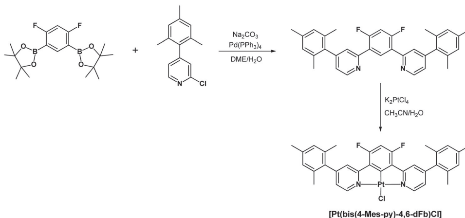
Scheme 1 Synthetic pathway for the preparation of [\text{Pt}(\text{bis}(4\text{-Mes-py})\text{-}4,6\text{-dFb})\text{Cl}] .
