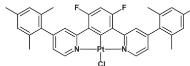
Chart 1 Investigated novel complex ([Pt(bis(4-Mes-py)-4,6-dFb)Cl]).
