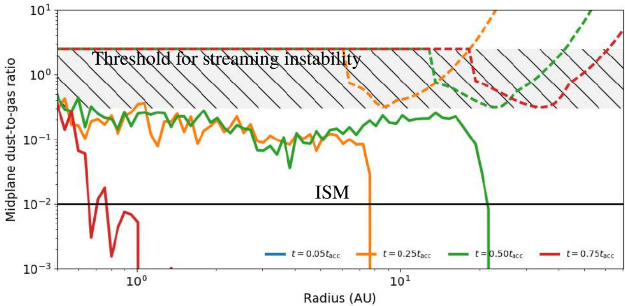
Fig. B.2. Midplane dust-to-gas ratios for the Std-Irg collapse model at the same time steps as shown in Figure B.1. The lines and hashed regions have the same definition as in Fig. 9.
