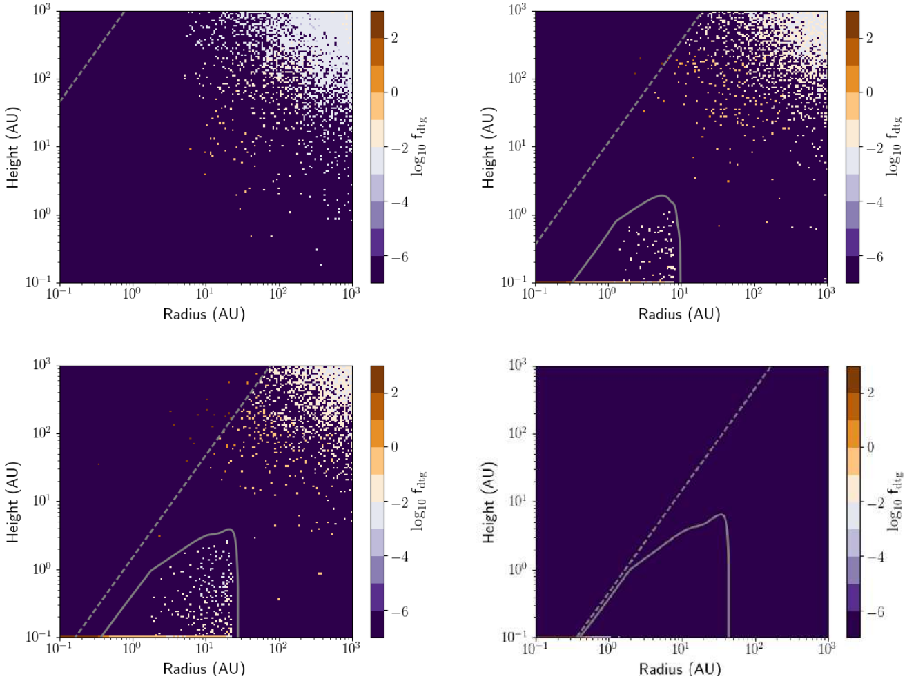
Fig. B.1. Same as Figure 8, but for the Std-Irg model. These larger grains evolve faster than the smaller grains. In particular, in the high density of the embedded disk, they radially drift very efficiently into the host star.
