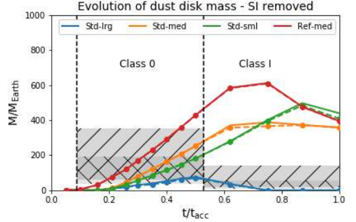
Fig. 13. Evolution of the dust mass, while removing the mass available for the streaming instability. In doing so, we can more closely match the class I disk masses found in the observations (grey regions, same as in Fig. 7). The Ref-med model finds almost no generation of planetesimals because dust mass in the disk midplane is very low (see Fig. 10).
