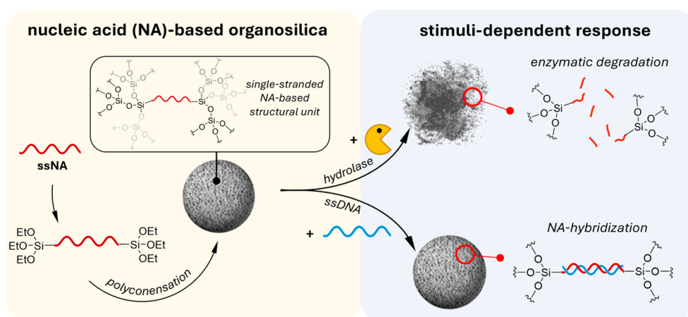
Figure 1. The presence of a covalently embedded nucleic acid (DNA or PNA) building block endows nucleic acid-based organosilica NPs with sequence-specific chemical, physical, and biological responsiveness.
