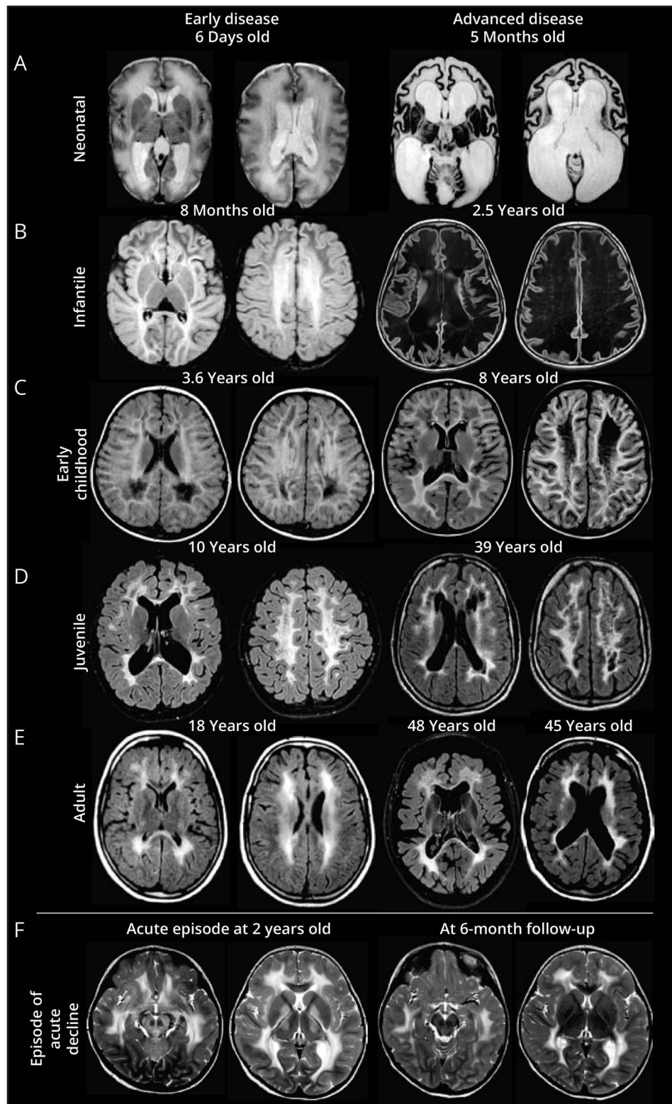
(A–E) Typical MRI findings per VWM subtype (increasing age at onset from top to bottom) and for early disease stage (left panel) or advanced disease stage (right panel) on T2 FLAIR images. A description of the corresponding MRI abnormalities is provided in Table 2. (F) Hyperintensities on T2-weighted images in the midbrain, basal ganglia, and thalami associated with an acute episode (left panel), which spontaneously resolved after 6 months (right panel). FLAIR = fluid-attenuated inversion recovery; VWM = vanishing white matter.
