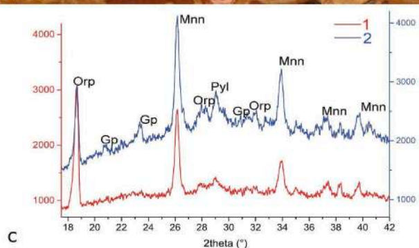
Fig. 11. Casket S.8212; detail of the left and right hieroglyphs with XRF (a) and XRD (c) data from point analysis (b). Mineral abbreviations in (c) are according to IMA–CNMNC: gypsum = gp, manganite = mnn, orpiment = orp, pyrolusite = pyl.
