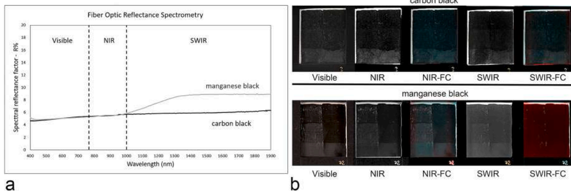
Fig. 2. a) Comparison of the spectral reflectance factors of the carbon black and manganese black showing a slight difference after 1400 nm; b) Comparison of black carbon and black manganese mock-ups in NIR and SWIR bands and the corresponding false color showing slight differences only in the SWIR band.
