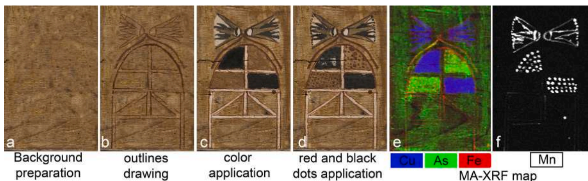
Fig. 5. Detail of the food cabinet of casket S. 8212, simulation of the scene realization steps: from the prepared wood (a) to the outlines of the structure and the lotus flower in red ochre (b); the white, blue, and red spots (c); the red and black dots applied as last decoration step on top. MA-XRF correlation map of Fe, As, Cu given as an RGB false color image (e); MA-XRF map of Mn (f).
