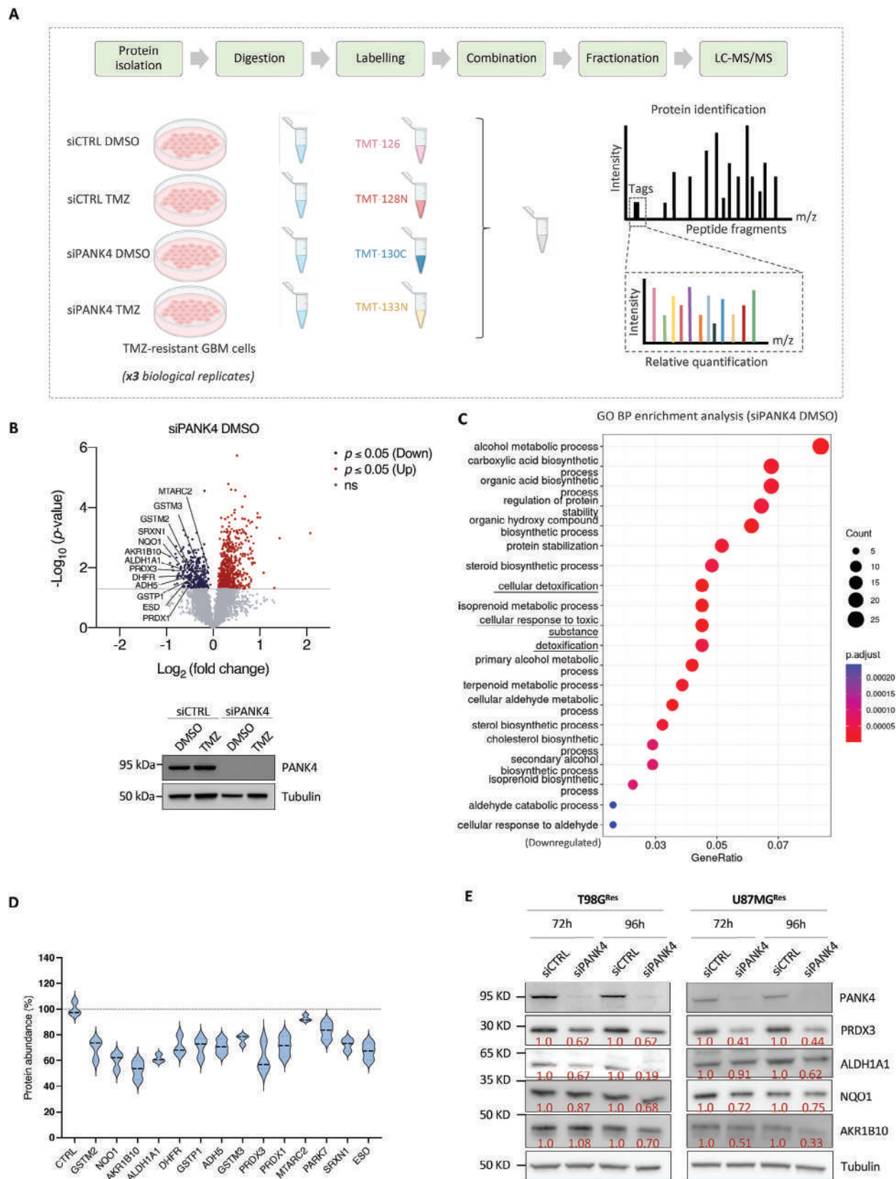
Figure 7. TMT-based proteomic analysis reveals reduced cell detoxification response upon PANK4 knockdown. A) Schematic representation of the Tandem Mass Tag (TMT) proteomic experiment. The following four conditions were assessed in T98G Res cells: siCTRL DMSO, siCTRL TMZ, siPANK4
