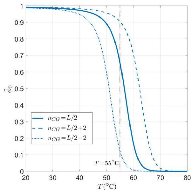
Figure 5. Dependence on the temperature T of the on-target primer pairing probability conditioned on the well-paired 3' end for PCR. Fixed values are considered for primer length L = 20 , salt concentration [Na^+] = 55 mM, and total sites L_0 = 6 \times 10^9 , for different CG fractions in the primer. Solid line: CG fraction n_{CG} = L/2 . Dashed line: CG fraction n_{CG} = L/2 + 2 . Dotted line: CG fraction n_{CG} = L/2 - 2 . The gray line marks T = 55^\circ\text{C} , a typical annealing temperature in the PCR experiments.
