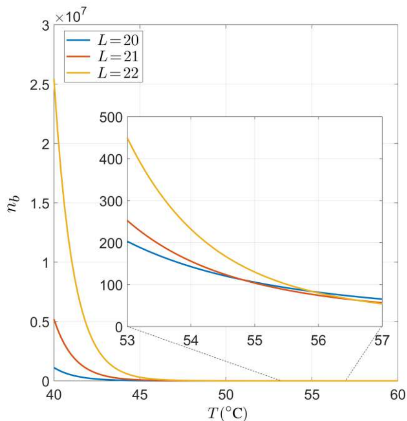
Figure A2. Dependence on the temperature T of the typical number of primers bounded per genome. We have considered fixed values for c_p = 400 nM, c_g = 0.4 fM, L_0 = 6 \times 10^9 , whereas we have considered L = 20 , L = 21 and L = 22 as typical primer lengths. The drop of n_b around the working temperature justifies the use of the approach used in the main text.
