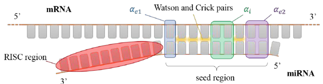
Figure 2. Sketch of a miRNA seed interacting with a generic portion of a mRNA. The nucleobases involved in the interaction with the AGO protein (red shading) are not available for pairing. Colored boxes have the same color code as Figure 1. In this sketch, \alpha_i = 2 , \alpha_{e1} = 1 and \alpha_{e2} = 2 .
