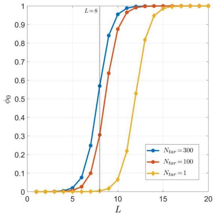
Figure 7. Dependence on the miRNA length L of the target pairing probability \phi_0 for fixed temperature T = 37\text{ }^\circ\text{C} , total sites L_0 = 1.1 \times 10^7 , salt concentration [Na^+] = 150\text{ mM} , and CG fraction n_{CG} = L/2 . Curves correspond to different numbers of distinct miRNA targets N_{tar} . Yellow dots: N_{tar} = 1 . Red dots: N_{tar} = 100 . Blue dots: N_{tar} = 300 . The gray line marks L = 8 , the typical length of the seed region of miRNA.
