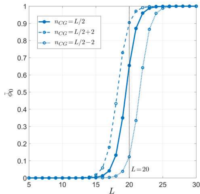
Figure 4. Dependence on the primer length L of the on-target pairing probability conditioned on the well-paired 3' end for PCR. Fixed values are considered for temperature T = 55^\circ\text{C} , salt concentration [Na^+] = 55\text{ mM} , and total sites L_0 = 6 \times 10^9 , for different CG fractions in the primer. Full dots and solid line: CG fraction n_{CG} = L/2 . Open dots and dashed line: CG fraction n_{CG} = L/2 + 2 . Open dots and dotted line: CG fraction n_{CG} = L/2 - 2 . Curves are computed using the average energetic description, detailed on the CG fraction (Equations (11) and (12)). The vertical gray line stands for L = 20 , a typical primer length in PCR.
