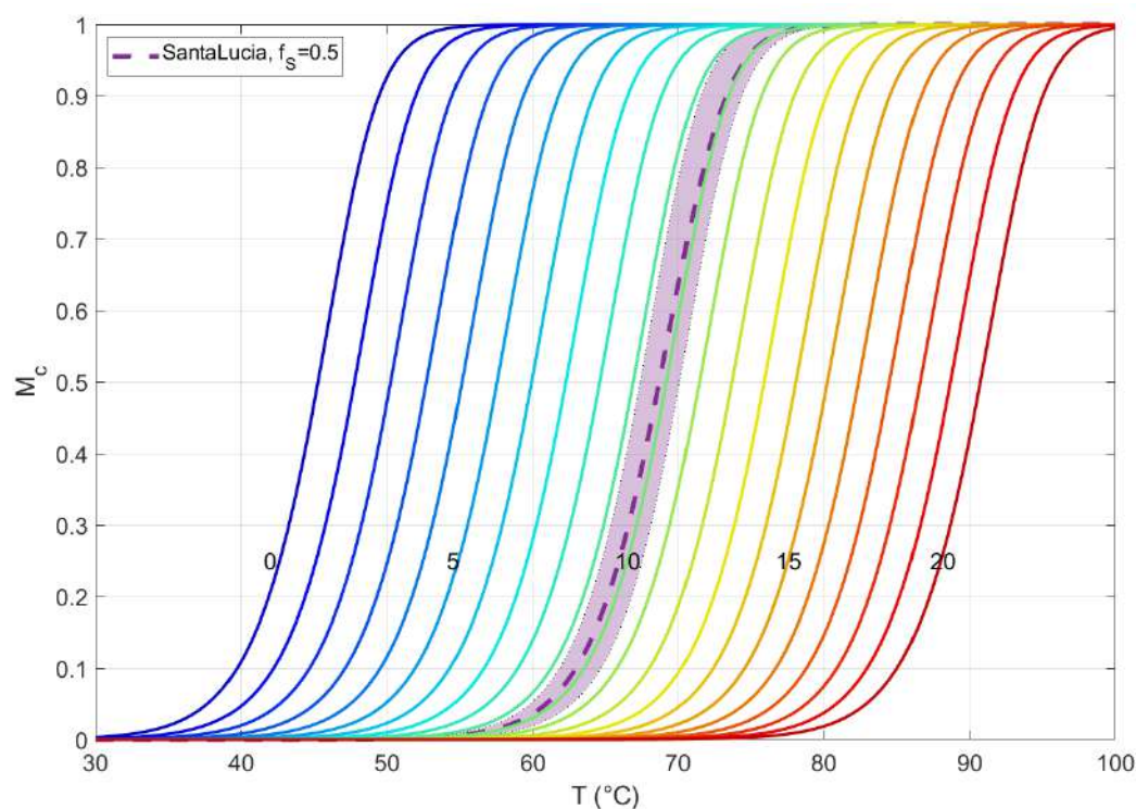
Figure A1. Melting curves of solutions of two 20 mers with perfect complementarity, computed with the analytical expression of a complementary system with two equipopulated species [11], with different pairing energies. The colored lines are computed with our averaged thermodynamic parameters, with number of C or G bases ranging from 0 to 20. Melting curves of 40 different duplexes with f_S = 0.5 have been computed with the energetic parameters obtained with the standard NN protocol for each duplex; the average of these melting curves and the standard deviation are represented in the purple dashed line and shadow, respectively. All the solutions are in the same experimental conditions: c_{DNA} = 100 nM and [Na^+] = 1 M.
