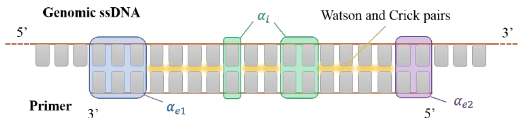
Figure 1. Sketch of a DNA primer interacting with a generic portion of a DNA single strand of a denaturated genome. Gray rectangles represent the nucleobases. Canonical Watson–Crick pairing is marked in yellow. Shaded boxes mark pairing defects: internal mismatches (green shades, counted by \alpha_i ), terminal mismatches at the 3' and 5' ends (blue shades, \alpha_{e1} and purple shades, \alpha_{e2} respectively). In this sketch, \alpha_i = 3 , \alpha_{e1} = 3 and \alpha_{e2} = 2 .
