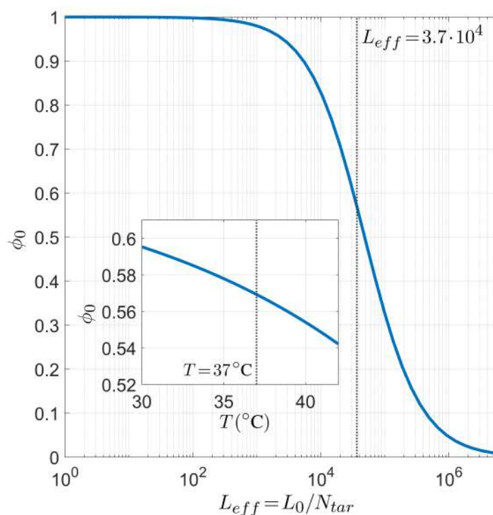
Figure 8. Dependence of the miRNA pairing probability \phi_0 on the reduced transcriptome length L_{eff} computed with N_{tar} = 300 for fixed temperature T = 37^\circ\text{C} , salt concentration [Na^+] = 150\text{ mM} , CG fraction n_{CG} = L/2 , and miRNA length L = 8 . Inset: T dependence of \phi_0 in the same conditions and L_{eff} = 3.7 \times 10^4 . The gray lines mark the reference values T = 37^\circ\text{C} (inset) and L_{eff} = 3.7 \times 10^4 (main figure).
