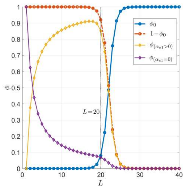
Figure 3. Dependence on the primer length L of the pairing probability for PCR. Fixed values are considered for temperature T = 55^\circ\text{C} , total sites L_0 = 6 \times 10^9 , salt concentration [Na^+] = 55\text{ mM} , and for CG fraction n_{CG} = L/2 . Successful target binding ( \phi_0 , blue dots). Off-target binding ( 1 - \phi_0 , red dots). Off-target binding can be split into 2 contributions: off-target binding with no terminal defects at the 3' end ( \phi_{(\alpha_{e1}=0)} , purple diamonds), off-target binding with terminal defects at the 3' end ( \phi_{(\alpha_{e1}>0)} , yellow diamonds). The vertical gray line stands for L = 20 , a typical primer length in PCR.
