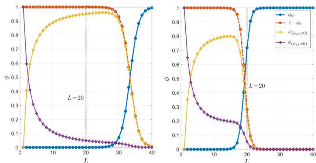
Figure A3. Dependence on the primer length L of the pairing probability for PCR. The plots are completely analogous to that shown in Figure 3 but with [Na^+] = 55/4 mM (left panel) and [Na^+] = 4 \times 55 mM (right panel).
