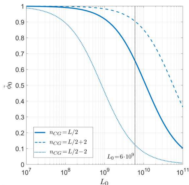
Figure 6. Dependence on the genome length L_0 of the on-target primer pairing probability conditioned on the well-paired 3' for PCR. Fixed values are considered for temperature T = 55^\circ\text{C} , salt concentration [Na^+] = 55\text{ mM} , and primer length L = 20 , for different CG fractions in the primer. Solid line: CG fraction n_{CG} = L/2 . Dashed line: CG fraction n_{CG} = L/2 + 2 . Dotted line: CG fraction n_{CG} = L/2 - 2 . The gray line marks twice the length of the human genome, L_0 = 6 \times 10^9 .
