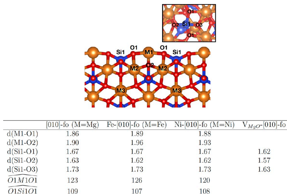
Figure 2. Side-view figure that shows the labels of the atomic positions of the [010]-fo forsterite. M shows the location of an Mg, Fe, and Ni atoms or MgO vacancy. The table reports distances ( d ), in Angstrom ( \text{\AA} ), and angles, in degrees ( ^\circ ), of the atoms found in the top figure.
