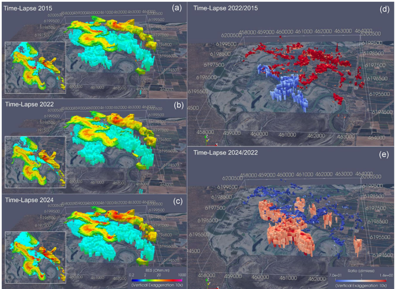
Figure 15. (a–c) Resistivity volumes extracted for the shallow part (Elevation > –25 m.a.s.l, Resistivity > 2 \Omega -m) and the deep part (Elevation < –25 m.a.s.l, Resistivity > 1.5 \Omega -m) from the 2015, 2022 and 2024 time-lapse models. The plan-view is shown in the bottom-left corner of each panel. (d, e) Volumes showing differences greater than \pm 8 per cent from the 2022/2015 and 2024/2022 ratio-models. Red colours indicate resistivity increases, and blue shows decreases.
