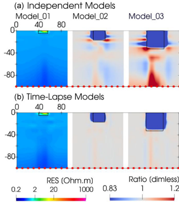
Figure 2. Synthetic test comparing independent and time-lapse schemes for inverting AEM temporal series. (a) Independent inversion models. (b) Time-lapse inversion models. From left to right in both (a) and (b), the true models simulate the growth of a high-resistivity anomaly with its true shape delineated by the overlaying black line. The models are shown over their DOI and the EM sounding positions are indicated at the bottom of each model (red dots).
