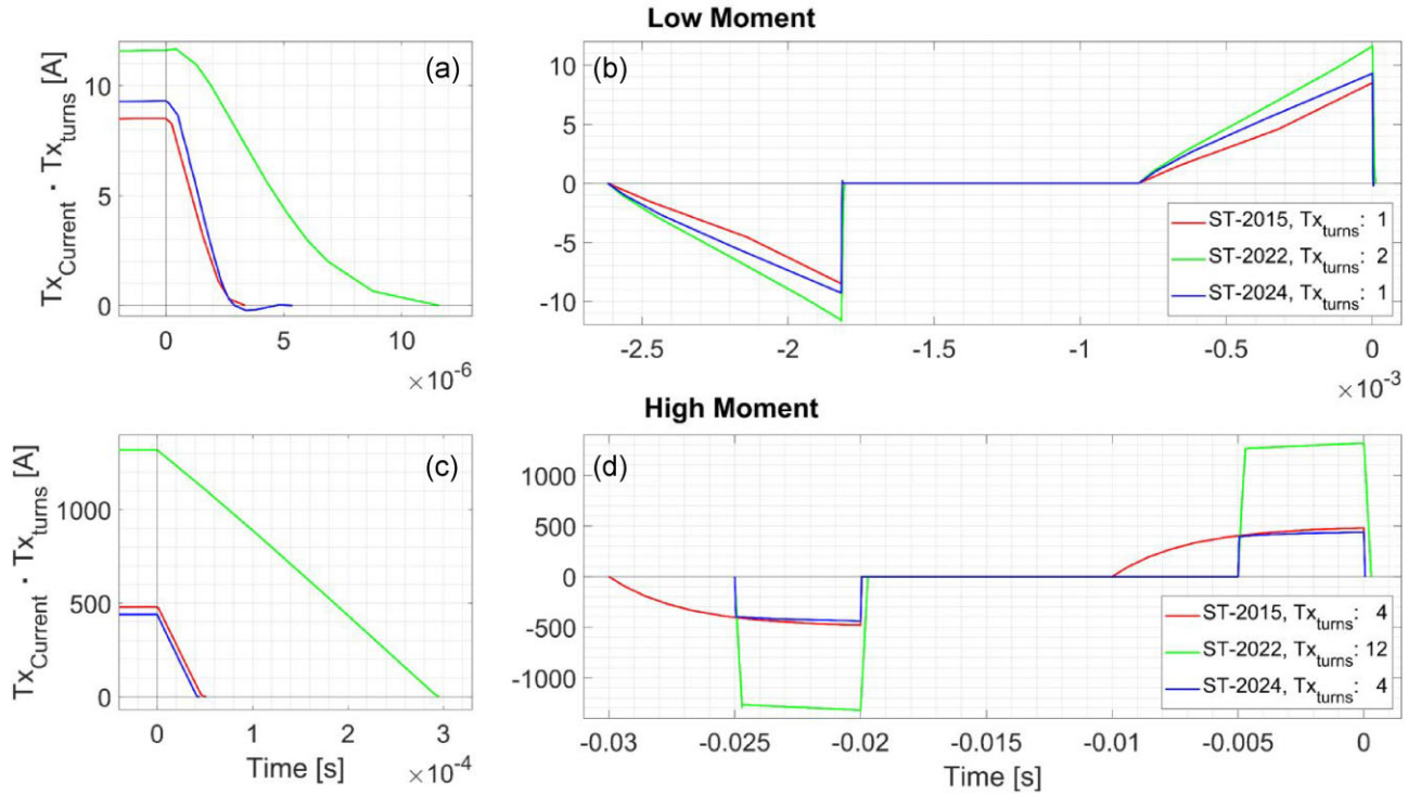
Figure 4. Energization characteristics of the SkyTEM systems used in the 2015 (red), 2022 (green) and 2024 (blue) Bookpurnong monitoring. The first row shows the low-moment energizations, highlighting the shut-down ramp (panel a) and a complete measuring cycle (panel b). The second row (panel c and d) details the high-moment energizations.
