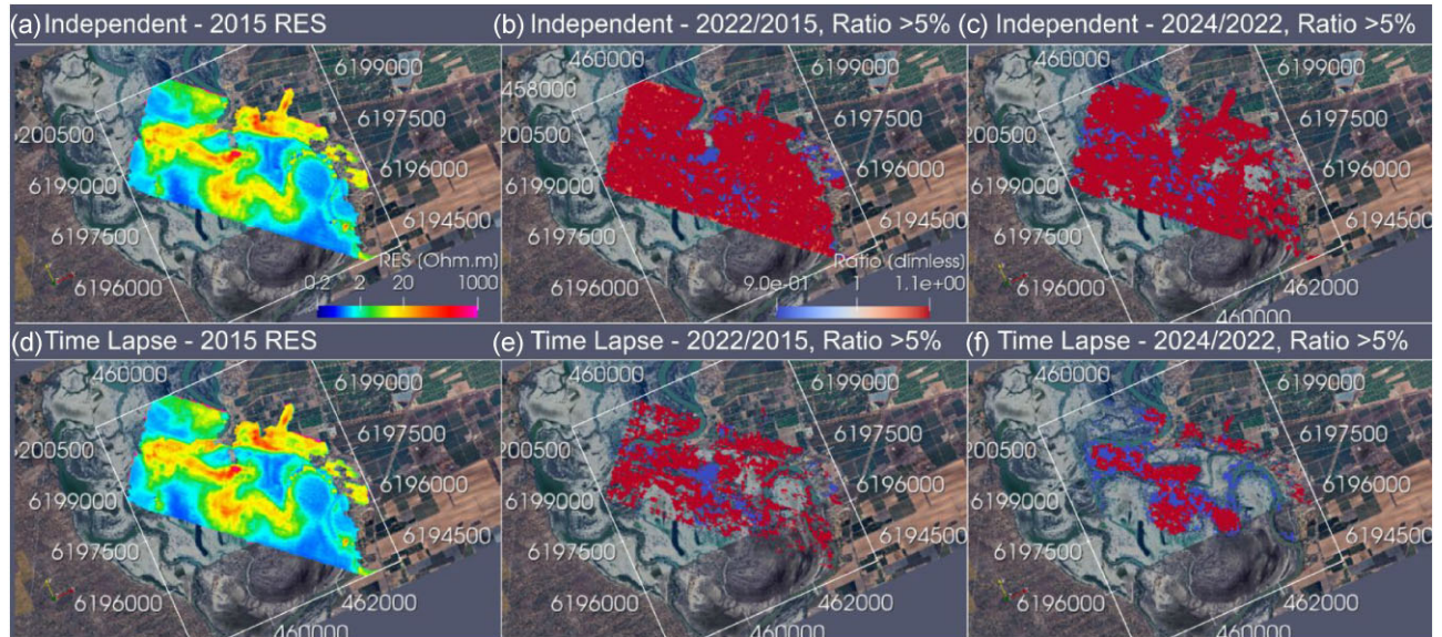
Figure 7. Real-case comparison of independent and time-lapse inversions performed on the Bookpurnong data sets. (a) 2015 resistivity model obtained through independent inversion. (b) Ratio of 2022 to 2015 independent resistivity models. (c) Ratio of 2024 to 2022 independent resistivity models. (d) 2015 resistivity model obtained through time-lapse inversion. (e) Ratio of 2022 to 2015 time-lapse resistivity models. (f) Ratio of 2024 to 2022 time-lapse resistivity models. All ratio model shows differences greater than \pm 5 per cent.
