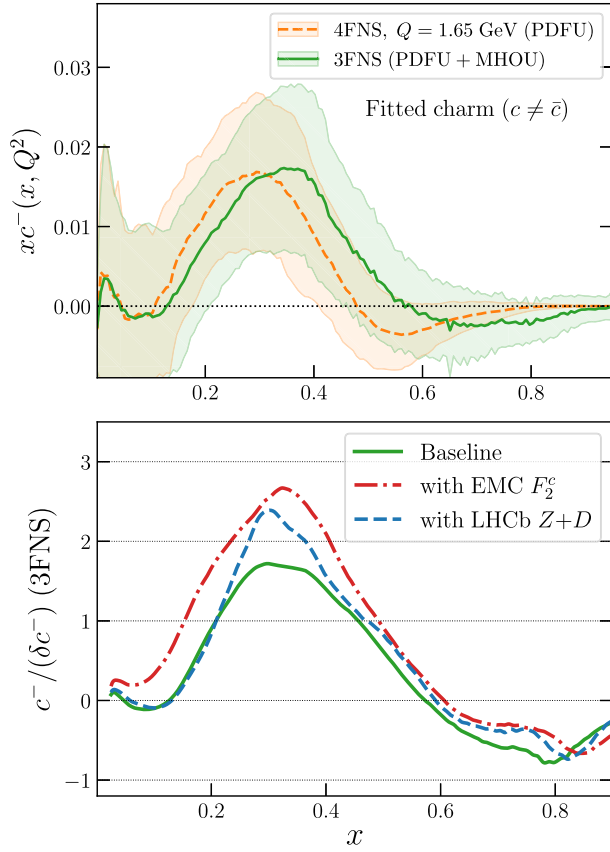
FIG. 3. Top: the 3FNS (intrinsic) valence charm PDF xc^- , compared to the 4FNS result (the same as Fig. 1 bottom). The 3FNS also includes MHOUs due to the inversion from the 4FNS to the 3FNS. Bottom: the pull for valence xc^- charm PDF in the 3FNS. Results are shown both for the default fit and also when including the EMC F_2^c and LHCb Z+c data.
