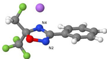
Fig. 1 Int-F molecule, in which the nitrogen atom near the oxygen in the oxadiazole ring is referred to as N2, as described in this section, whereas the nitrogen at position 4, coordinated with the Li atom (pink), is referred to as N4.
