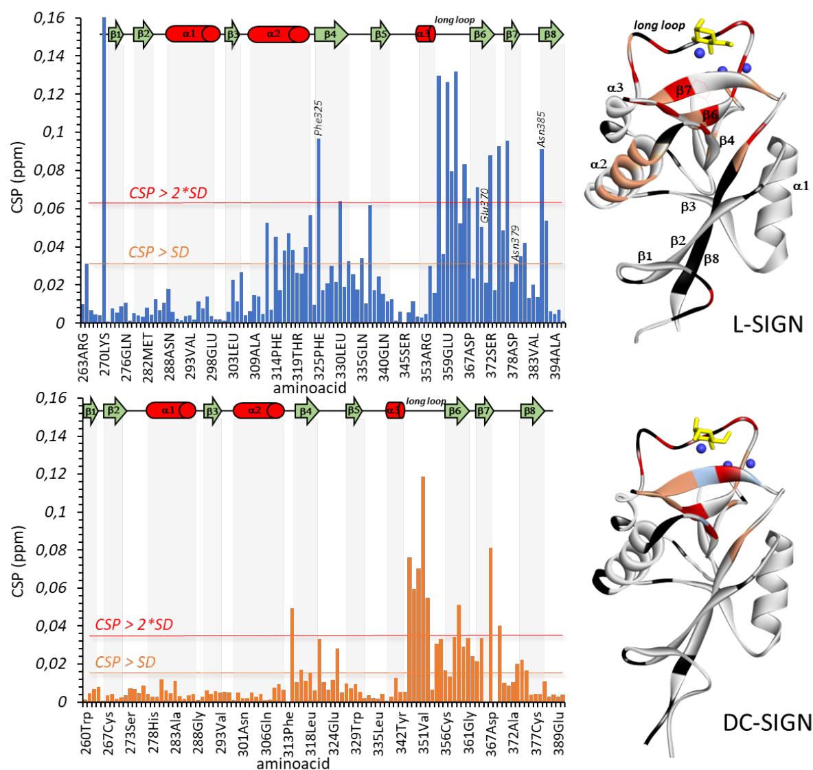
Figure 5. The binding of Man84 to L-SIGN (top) and DC-SIGN (bottom) in solution, by monitoring NMR signals of the corresponding protein in the absence and presence of the ligand (30 equivalents in the case of L-SIGN, and 100 equivalents for DC-SIGN). On the left, plots for the CSP analysis (average chemical shift difference between protein free and bound states, as described in the experimental section) and on the right 3D cartoon representation of the corresponding protein highlighting the most affected residues in the CSP analysis: in red residues with CSP above twice the standard deviation (SD) of the whole data set, and orange residues with CSP above the SD. Residues in black are not assigned or are Prolines. Residues in light blue disappear in the bound state. The ligands are in yellow and \text{Ca}^{2+} ions in dark blue. For L-SIGN, residues involved in direct intermolecular interactions with Man84 as found by X-ray crystallography are annotated in the CSP plots.
