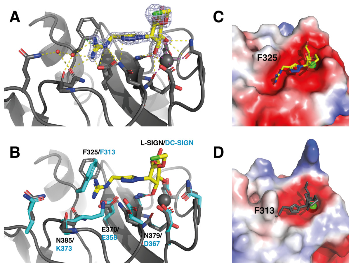
Figure 4. 3D structural binding mode of Man84 within L-SIGN CRD and mechanism of selectivity. (A) Structure of the L-SIGN CRD/ Man84 complex (PDB: 8RCY). Man84 is shown superimposed over the Fo-Fc electron density map (light blue, 2\sigma contour) within L-SIGN CRD. Side chain of residues involved in the binding are represented as sticks. H-Bond are represented as yellow dashed lines, \text{Ca}^{2+} coordination bond as magenta dashed line and \pi -cation interaction by green dashed lines. Water molecules are represented as red spheres. (B) Alignment with the CRD of DC-SIGN (PDB: 2IT6) for comparative purposes. Side chain of corresponding residue from DC-SIGN CRD are presented as cyan sticks and labelled. Electrostatic surfaces of L-SIGN CRD (C) and DC-SIGN CRD (D) were calculated via the PyMol software, with complexed Man84 represented in yellow in L-SIGN CRD or in grey in DC-SIGN CRD where it has been added by structural alignment for comparison. The \text{Ca}^{2+} ion in the binding site is represented by a grey sphere. (see Table S1 for data collection and structure refinement statistics).
