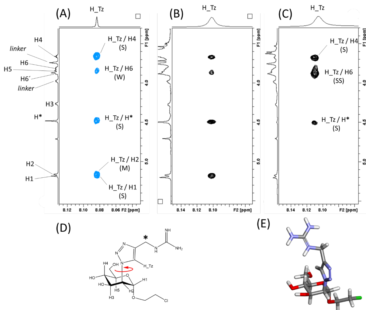
Figure 6. The binding of Man84 to DC-SIGN and L-SIGN in solution from the ligand perspective. Blue contours correspond to positive NOE, while black contours correspond to negative NOE. (A) NOESY spectrum of Man84 showing the positive NOE correlations of H_Tz. (B) The same region of the trNOESY spectrum of Man84 in the presence of DC-SIGN (1:17 protein:ligand molar ratio). (C) The same region of the trNOESY spectrum of Man84 in the presence of L-SIGN (1:10 protein:ligand molar ratio). (D) Structure of Man84 showing the free rotation around the C2(Man)-N(Triazol) bond. (E) The L-SIGN-bound conformation of Man84 , as derived by NMR interaction data. This conformation corresponds to the one observed in the X-ray structure (Fig. 4A).
