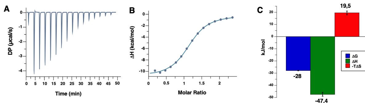
Figure 3. Titration of the Man84 ligand at 2 mM to L-SIGN ECD (172 \mu\text{M} ) by ITC. (A) Representative data among a series of 3 of the titration thermograms obtained (see Supp. info for all ITC titration experiments). (B) Data integration with fitted curve, using 1:1 binding model. (C) Average thermodynamic parameters values obtained following the L-SIGN CRD/ Man84 complex formation.
