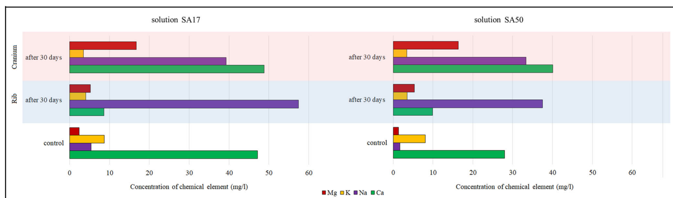
FIGURE 1 Concentrations of the major elements in the solutions analyzed before and after the aging, provided by the MP-AES. [Colour figure can be viewed at wileyonlinelibrary.com ]
