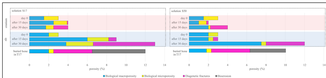
FIGURE 4 Graphical representation of the fractions of biological and diagenetic porosity with respect to the total porosity reported for each aged and buried bone analyzed (e.d.s. 10%). [Colour figure can be viewed at wileyonlinelibrary.com ]
