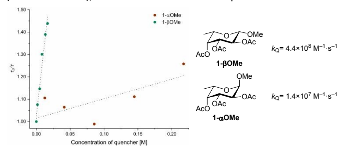
Fig. 5 Stern-Volmer plots and quenching constants for 1- \beta OME and 1- \alpha OME measured at 25 °C in MeCN.
