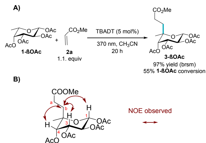
Fig. 3 A) TBADT promoted Giese-type alkylation of \beta -tetra- O -acetylucose 1- \beta OAc with methyl acrylate 2a . Isolated yield of 3- \beta OAc based on consumed 1- \beta OAc ; B) NOESY experiments allowed to establish the C-5 configuration of 3- \beta OAc .
