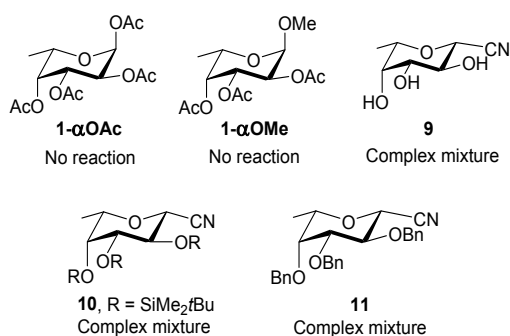
Chart 1 Control reactions on substituted fucosides (0.1 M) under TBADT photocatalyzed conditions in the presence of 2a (1.1 equiv.).
