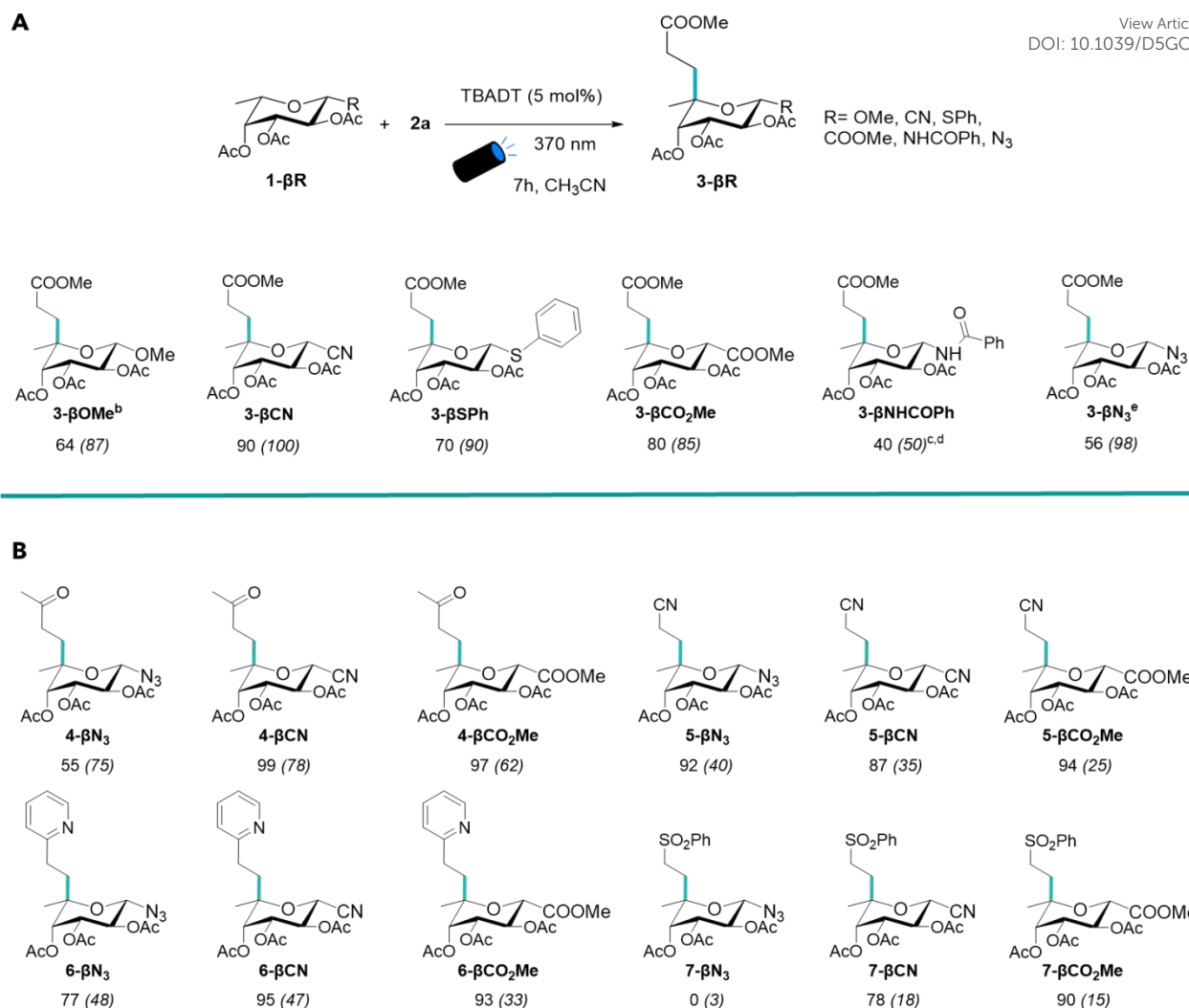
Fig. 4 Scope of: A) \beta -Fucosides and B) Alkenes. a Reaction conditions: 1- \beta R (1 equiv, 0.1 M), methyl acrylate 2a (1.1 equiv), TBADT (5 mol%) under 370 nm irradiation in MeCN for 7 h. The C-5 configuration of all products was established by NOESY experiments. 3- \beta R Isolated yield brsm and ( 1- \beta R % conversion) are reported. Conversions were determined by 1 H-NMR of the crude reaction mixtures. b Alkylated by-product on OMe was also formed (10% yield); c 20 h irradiation; d Yields were estimated by 1 H-NMR analysis of the crude reaction mixture since 3- \beta NHCOPh was inseparable from the remaining 1- \beta NHCOPh ; e 3 h irradiation. An oligomeric adduct was also formed in 12% yield).
