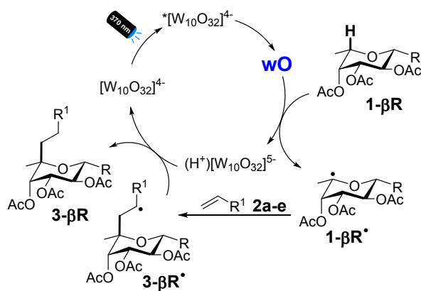
Scheme 2 Mechanistic proposal.
