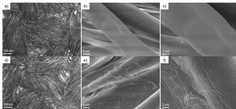
Figure 2. SEM micrographs at different magnifications of: (a–c) untreated cotton (250 \times , 5000 \times and 10,000 \times ) and (d–f) cotton fabrics treated with 8% add-on M-PCASS (250 \times , 5000 \times and 10,000 \times ).
