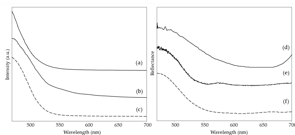
Figure 8. (Left) Emission spectra ( \lambda_{exc} = 435 nm) of blue areas: (a) The grammar of fire—Canto II , area 1, (b) The North star and the tree of life , area 3, (c) reference sample of B029. (Right) Visible reflectance spectra of blue areas: (d) The grammar of fire—Canto II , area 1, (e) The North star and the tree of life , area 3, (f) reference sample of B029. Legend: (solid lines) spectra acquired on the paintings; (dashed lines) spectra of reference fluorescent paints.
