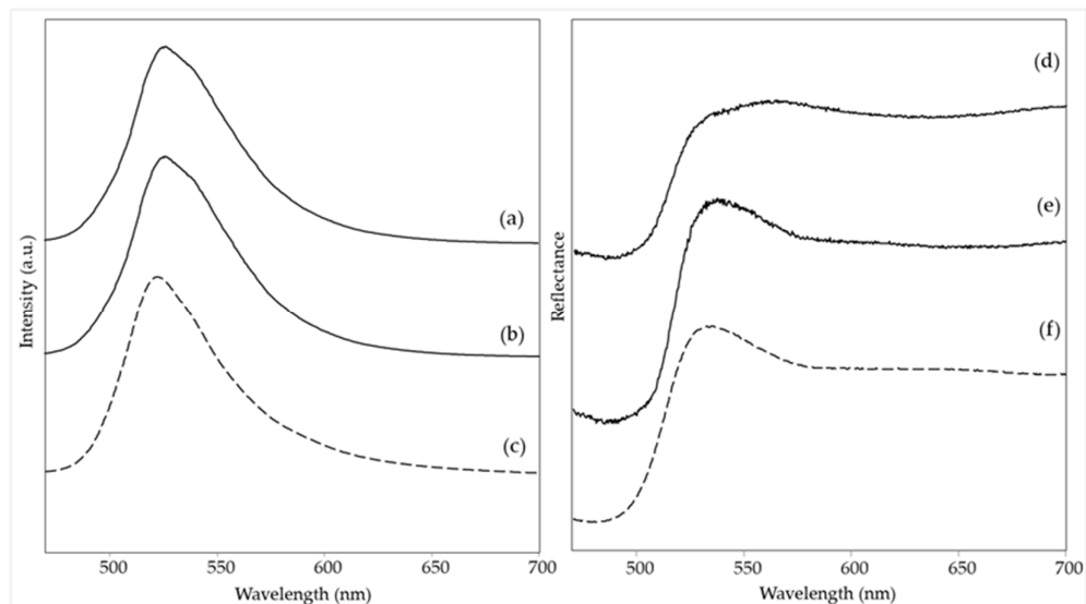
Figure 4. (Left) Emission spectra ( \lambda_{exc} = 435 nm) of yellow areas: (a) The North pole and the tree of life , area 5, (b) Earthquake , area 2 and (c) reference sample of Y173. (Right) Visible reflectance spectra of yellow areas: (d) The North pole and the tree of life , area 5, (e) Earthquake , area 2, and (f) reference sample of Y173. Legend: (solid lines) spectra acquired on the paintings; (dashed lines) spectra of the reference fluorescent paint.
