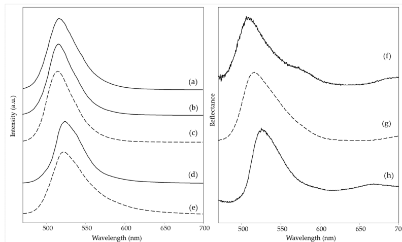
Figure 6. (Left) Emission spectra ( \lambda_{\text{exc}} = 435 \text{ nm} ) of green areas: (a) The grammar of fire—Canto I , area 2, (b) The North star and the tree of life , area 4, (c) reference sample of G590, (d) Earthquake , area 3 and (e) reference sample of Y173. (Right) Visible reflectance spectra of green areas: (f) The North star and the
