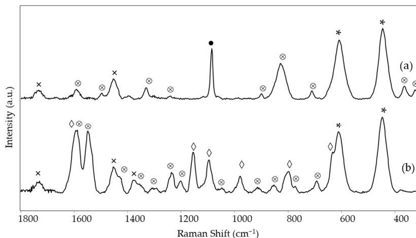
Figure 3. SSE™ Raman spectra of yellow areas: (a) The North pole and the tree of life , area 5 and (b) Earthquake , area 2. Legend: ⊗ = pigment (for wavenumbers and assignments see Table 2), * = rutile, • = \text{CaCO}_3 , ◊ = resin, × = binder (see text).
