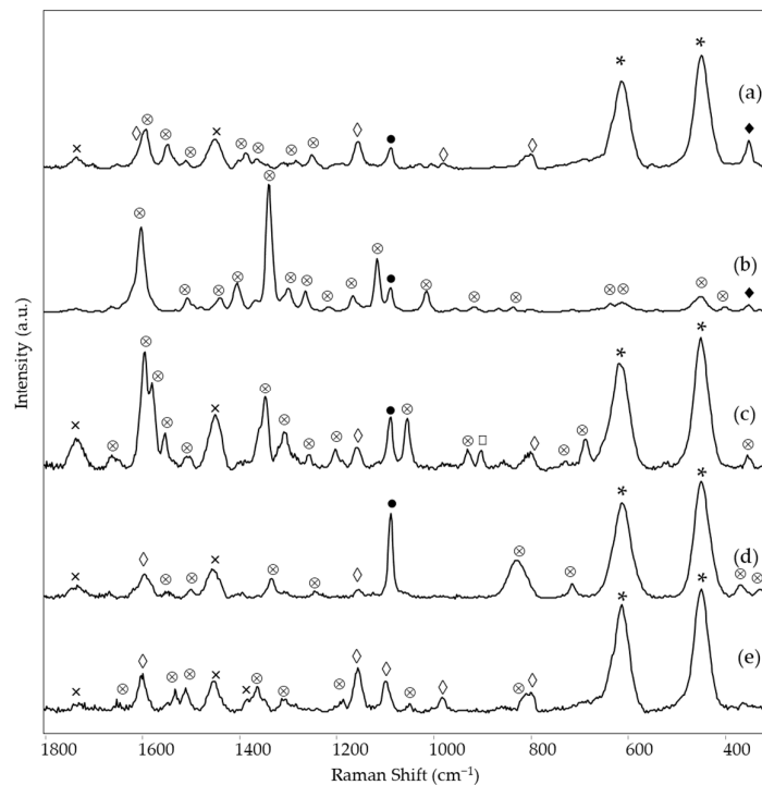
Figure 1. SSE™ Raman spectra of red areas: (a) The grammar of fire—Canto I , area 1, (b) The grammar of fire—Canto II , area 2, (c) The North star and the tree of life , area 1, (d) The North star and the tree of life , area 6 (orange) and (e) Earthquake , area 1. Legend: ⊗ = pigment (for wavenumbers and assignments see Table 2), * = rutile, • = \text{CaCO}_3 , ◇ = resin, □ = \text{Sr}_2\text{MgSi}_2\text{O}_7 , ◆ = ZnS, × = binder (see text).
