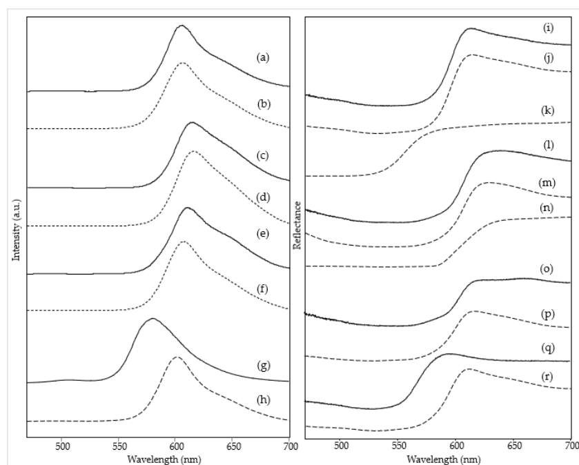
Figure 2. (Left) Emission spectra ( \lambda_{\text{exc}} = 435 \text{ nm} ) of red areas: (a) The grammar of fire—Canto II , area 2, (b) reference sample of R371, (c) The North star and the tree of life , area 1, (d) reference sample of R435, (e) Earthquake , area 1, (f) reference sample of R376, (g) The North star and the tree of life , area 6 and (h) reference sample of O232. (Right) Visible reflectance spectra of red areas: (i) The grammar of fire—Canto II , area 2, (j) reference sample of R371, (k) reference sample of PO62, (l) The North star and the tree of life , area 1, (m) reference sample of R435, (n) reference sample of PR254, (o) Earthquake , area 1, (p) reference sample of R376, (q) The North star and the tree of life , area 6 and (r) reference sample of O232. Legend: (solid lines) spectra acquired on the paintings; (dashed lines) spectra of reference fluorescent paints or conventional pigments. Grey line—black line
