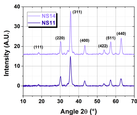
Fig. 3 XRD patterns of the NS11 and NS14 magnetic cores.
