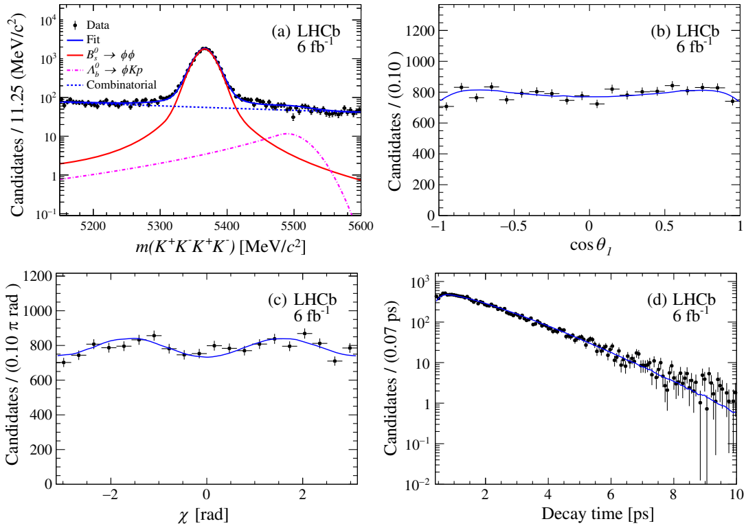
FIG. 1. (a) Mass distribution of the B_s^0 \rightarrow \phi\phi candidates, superimposed by the fit projections. (b)–(d) Background-subtracted distributions of angular variables ( \cos \theta_1 and \chi ) and decay time, superimposed by the fit projections.
