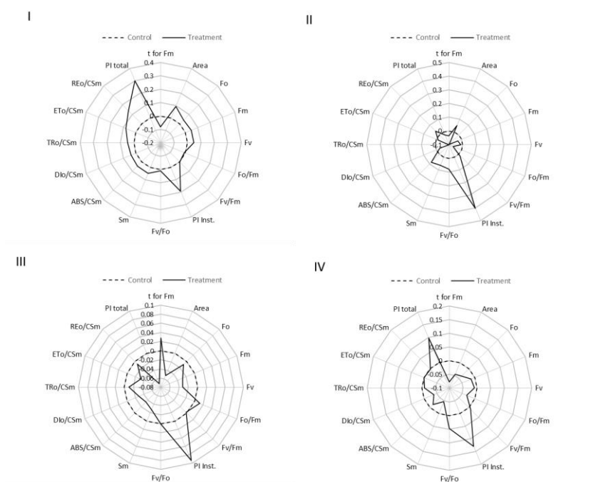
Figure 3. Chlorophyll a fluorescence parameters measured in vivo in red (Codex) lettuce leaves. Measurements were taken 2 days after the first (I), the second (II), the third (III) application, and at harvest (IV). Values are means \pm SE ( n = 6 ). (F_t - F_c)/F_c , was used to normalize the data. In the formula, “ F_t ” and “ F_c ” represent the values of treated plants and control plants treated with water, respectively. Values of “ F_c ” plants were normalized to 0 (control plants treated with water, dotted line circle = 0).
