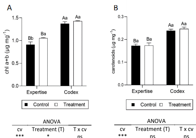
Figure 4. Chlorophyll a + b (A) and Carotenoids (B) concentration in green (Expertise) and red (Codex) lettuce leaves cultivars. Measurements were taken at harvest. Values are means \pm SE ( n = 4 ). The mean is subjected to a two-way ANOVA. Different uppercase and lowercase letters indicate significant differences between varieties and treatment, respectively, at p < 0.05 . ns, *, *** means not significant or significant at p < 0.05 and 0.001 , respectively.
