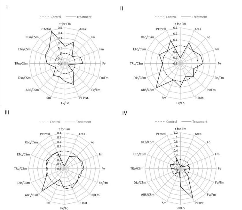
Figure 2. Chlorophyll a fluorescence parameters measured in vivo in green (Expertise) lettuce leaves. Measurements were taken 2 days after the first (I), the second (II), the third (III) application, and at harvest (IV). Values are means \pm SE ( n = 6 ). (F_t - F_c)/F_c , was used to normalize the data. In the formula, “ F_t ” and “ F_c ” represent the values of treated plants and control plants treated with water, respectively. Values of “ F_c ” plants were normalized to 0 (control plants treated with water, dotted line circle = 0).
