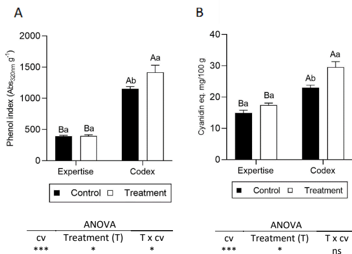
Figure 5. Phenol index (A) and Anthocyanin (B) concentration in green (Expertise) and red (Codex) lettuce leaves cultivars. Measurements were taken at harvest. Values are means \pm SE ( n = 4 ). The mean is subjected to a two-way ANOVA. Different uppercase and lowercase letters indicate significant differences between varieties and treatment, respectively, at p < 0.05 . ns, *, *** means not significant or significant at p < 0.05 and 0.001 , respectively.
