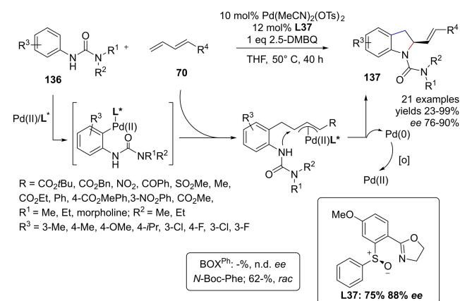
Scheme 66. Domino reaction of aryl ureas 136 in the presence of dienes 70 , yielding chiral 2-vinyl–indolines 137 .
