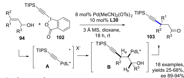
Scheme 48. Selective anti -Markovnikov addition of aryl boronic acids to yield 1,2-diaryl carbonyl compounds 100 .
