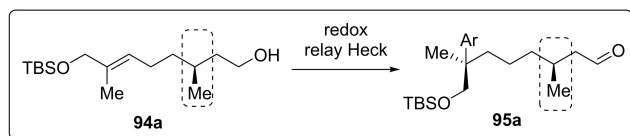
Scheme 45. Redox-relay Heck strategy for the enantio- and diastereoselective synthesis of quaternary stereocenter in compound 95 .
