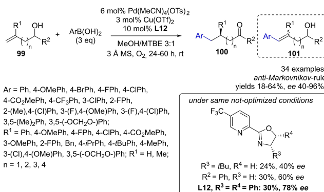
Scheme 48. Selective anti -Markovnikov addition of aryl boronic acids to yield 1,2-diaryl carbonyl compounds 100 .
