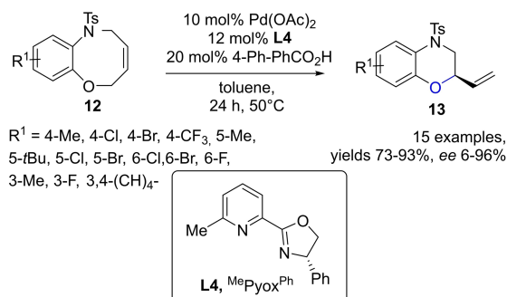
Scheme 7. Ring contraction of 12 as route to access 1-vinyl substituted benzooxazine 13 .
