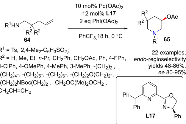
Scheme 30. Aminoacetoxylation of aminoalkenes 64 in the presence of the novel ligand L17 .
