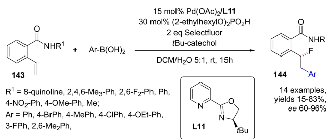
Scheme 70. Pd(II)-catalyzed asymmetric fluorination of styrenes 143 .
