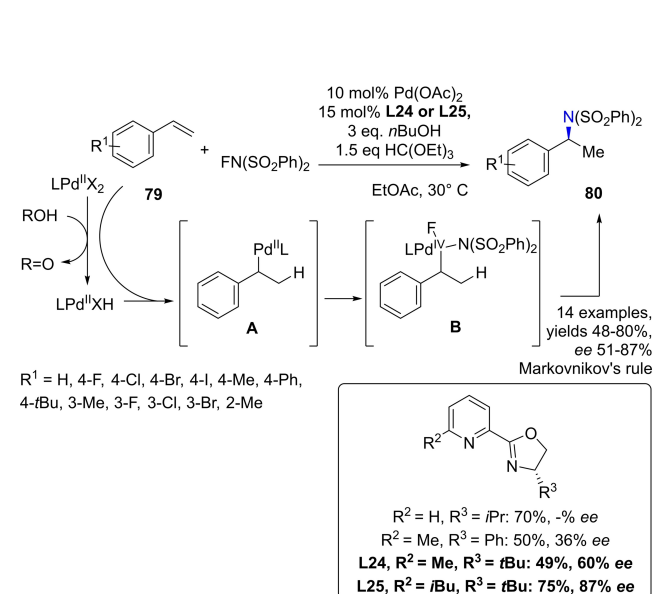
Scheme 38. Enantioselective hydroamination of styrenes 79 in the presence of NFSI as oxidant and nucleophilic source.
