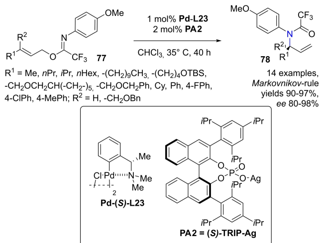
Scheme 37. ACDC driven by ( S )-TRIP–Ag in the presence of palladacycle L23 for the allylic rearrangement of acetimidates 77 .
