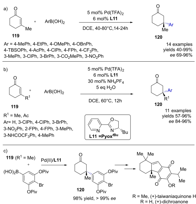
Scheme 57. Enantioselective addition of aryl boronic acids to \alpha,\beta -unsaturated cyclic ketones 119 as route to access tricyclic terpenoids.
