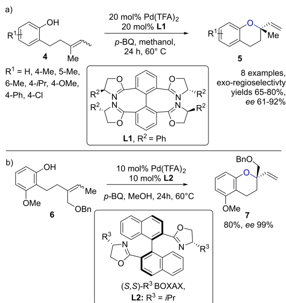
Scheme 4. Enantioselective synthesis of vinyl chromans 5 and 7 .
