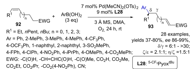
Scheme 44. Asymmetric arylation of alkenes 92 with β-hydride elimination driven by EWG located at (-CH 2 ) n distance.
