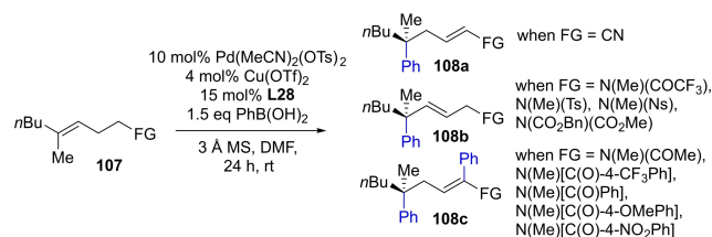
Scheme 51. Summary of the different outcomes investigated in function of the FG located at (-CH_2-)_2 distance from the olefin.
