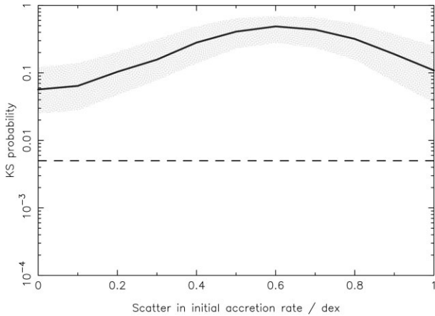
Figure 8. Probability that the observed accretion rates from Manara et al. (2022) are drawn from the same underlying distribution as our wind-driven model (equation (6)), as a function of the scatter in the initial accretion rate. As in Figs 5 and 7, the line represents the median from 1000 random realizations of the KS test, while the shared area spans the 25th to 75th percentiles of the distribution. The dashed horizontal line again marks a probability of 0.5 per cent. Although the probability peaks at a scatter of \simeq 0.6 dex, none of the parameter space for the wind-driven models is ruled out.
