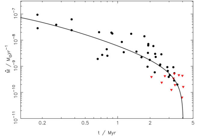
Figure 3. Simulated data generated for a model with \gamma = 1 , \dot{M}_c = 10^{-9} M_{\odot} \text{ yr}^{-1} , and \Delta_M = 0.35 . The solid curve shows the analytic form of \dot{M}(t) , and the points show the N = 50 simulated ‘observations’ generated from this curve, using the procedure described in Section 2.4. Black circles represent detections; red triangles represent upper limits.
