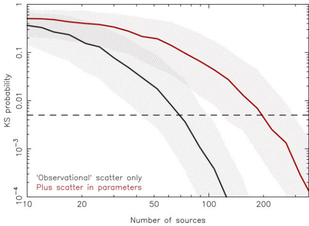
Figure 5. Probability that samples of accretion rates from the two different disc models could have been drawn from the same underlying distribution, as a function of the sample size N . Black/grey represents the ‘basic’ models, with only observational scatter in \dot{M} , while red denotes the results with significant scatter applied to all the input parameters. For each value of N , the Kolmogorov–Smirnov (KS) test was repeated for 1000 different random realizations of the models; the lines represent the median KS probability, while the shaded areas span the 25th to 75th percentiles of the distribution. The dashed horizontal line marks a probability of 0.5 per cent. For the basic model N \gtrsim 100 is sufficient to distinguish between viscous and wind-driven accretion, but with scatter applied to the input parameters the required sample size rises to N \gtrsim 300 .
