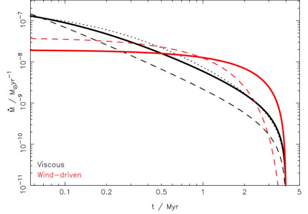
Figure 1. Accretion rate as a function of time in the canonical viscous (black line; equation (5)), and wind-driven (red line; equation (6)) disc models. The viscous model is essentially a power-law, truncated below the cut-off rate \dot{M}_c , so most of the disc lifetime is spent at low accretion rates. By contrast, in the wind-driven model accretion declines geometrically, so most of the disc lifetime is spent at high accretion rates, close to the initial value \dot{M}_0 . The dashed and dotted lines show the effect of varying different model parameters (while keeping M_{d,0} and the disc lifetime fixed). The dashed black line shows a viscous model with a lower cut-off accretion rate ( \dot{M}_c = 3 \times 10^{-10} M_\odot \text{yr}^{-1} ), while the dotted black line shows a model with power-law index \gamma = 3/2 . The dashed red line denotes a wind-driven model with \omega = 0.2 (which for a fixed disc lifetime also increases the initial accretion rate \dot{M}_0 ).
