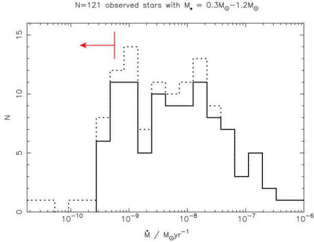
Figure 6. Distribution of observed accretion rates from the compilation of data in Manara et al. (2022): the solid line shows only detections, while the dashed histogram shows both detections and upper limits. We restrict our analysis to the traditional ‘T Tauri star’ range in stellar mass, defined here as 0.3\text{--}1.2 M_{\odot} , which results in a sample of 121 sources. However, modest changes in the range of stellar masses we consider do not change the distribution significantly. The red arrow denotes the detection threshold, \dot{M}_1 , applied to our simulated data (as described in Section 2.4.).
