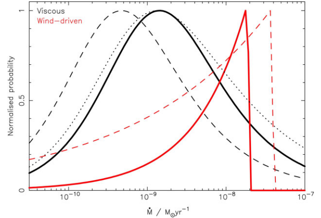
Figure 2. Accretion rate probability distributions p(\dot{M}) for the two disc models, assuming uniform sampling of \dot{M}(t) . As in Fig. 1, the solid black line represents the viscous model, and the solid red line the wind-driven model. For the viscous model the distribution peaks close to the cut-off rate \dot{M}_c , and is approximately symmetric around this peak. By contrast, the distribution for the wind-driven model always peaks at the initial (maximum) accretion rate \dot{M}_0 , and declines to smaller values. As in Fig. 1, the dashed and dotted curves show the effect of changing the model parameters. In the viscous model, lowering the cut-off rate \dot{M}_c shifts the peak of the distribution to lower \dot{M} by the same factor, while changing the power-law index \gamma has only a minor impact. In the wind-driven model, a lower value of the dissipation parameter \omega results in a broader distribution, and also shifts the peak to higher \dot{M} (as for a fixed disc lifetime, \dot{M}_0 \propto t_{\text{acc},0}^{-1} \propto \omega^{-1} ).
