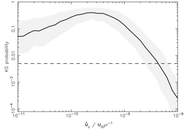
Figure 7. Probability that the observed accretion rates from Manara et al. (2022) are drawn from the same underlying distribution as our viscous model (equation (5)), as a function of the cut-off accretion rate \dot{M}_c . As in Fig. 5, the line represents the median from 1000 random realizations of the KS test, while the shaded area spans the 25th to 75th percentiles of the distribution. The dashed horizontal line again marks a probability of 0.5 per cent. We see that values of \dot{M}_c > 5 \times 10^{-9} M_{\odot} \text{ yr}^{-1} are strongly ruled out by our analysis: if photoevaporation terminates disc accretion, then the photoevaporative mass-loss rates must be low.
