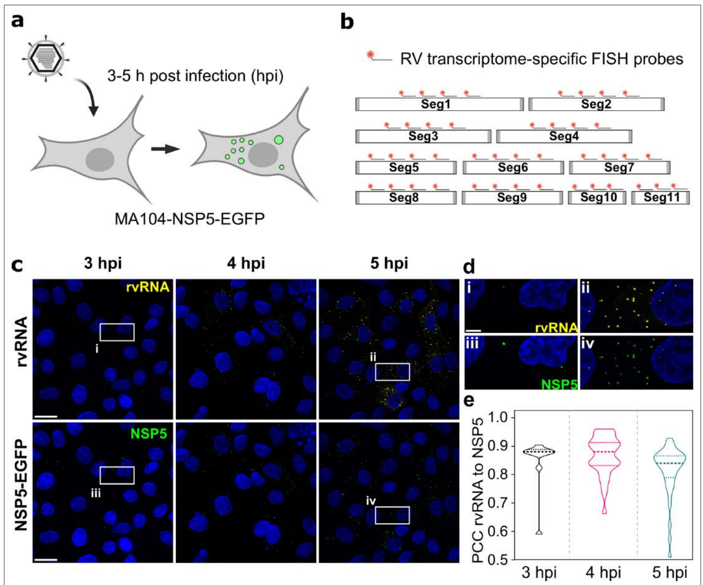
Figure 1. RNA accumulation during Rotavirus infection. (a) Experimental design for detecting EGFP-tagged viroplasm during early infection (3–5 hpi) stages. (b) Schematics of the FISH probe design for detecting all 11 RV transcripts. A pooled set of 3–4 segment-specific probes labelled with Quasar570 dye were used for visualising RV transcripts in EGFP-tagged viroplasm. (c) RV RNA accumulation in viral factories during early infection. Top: RV transcripts (yellow) visualized by smFISH using a combined set of 3–5 segment-specific probes targeting each genomic transcript. Bottom: NSP5-EGFP-tagged viral factories (green). Images represent maximum intensity Z-projections acquired using identical settings and brightness levels for both channels. DAPI-stained nuclei are shown in blue. Scale bars, 25 \mu m. (d) RV transcripts and NSP5-EGFP-specific signals shown in the white box in panel (c). Note the low intensity of the RNA and EGFP signals during early infection stages that increase by 5 hpi. Scale bar, 5 \mu m. (e) Pearson's correlation coefficients (PCCs) of colocalising NSP5-EGFP-tagged viral factories and RV transcripts, as shown above in panel (d). Dashed and dotted lines represent median and quartile values of PCCs, respectively. Each data point represents the PCC value calculated for a single cell. N=10 (3 hpi), N=31 (4 hpi), N=38 (5 hpi).
