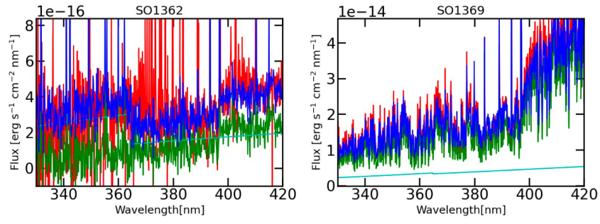
Fig. D.5. Best fit for the Balmer continuum region for targets in the \sigma -Orionis cluster, ordered by source name. - continued
