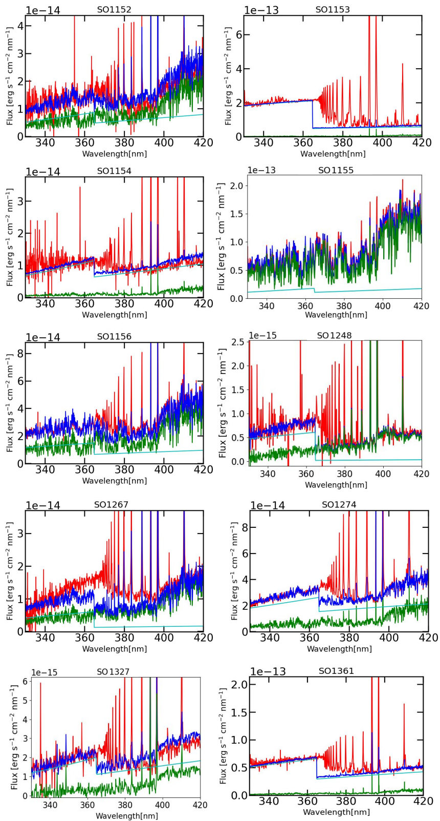
Fig. D.4. Best fit for the Balmer continuum region for targets in the \sigma -Orionis cluster, ordered by source name. - continued
