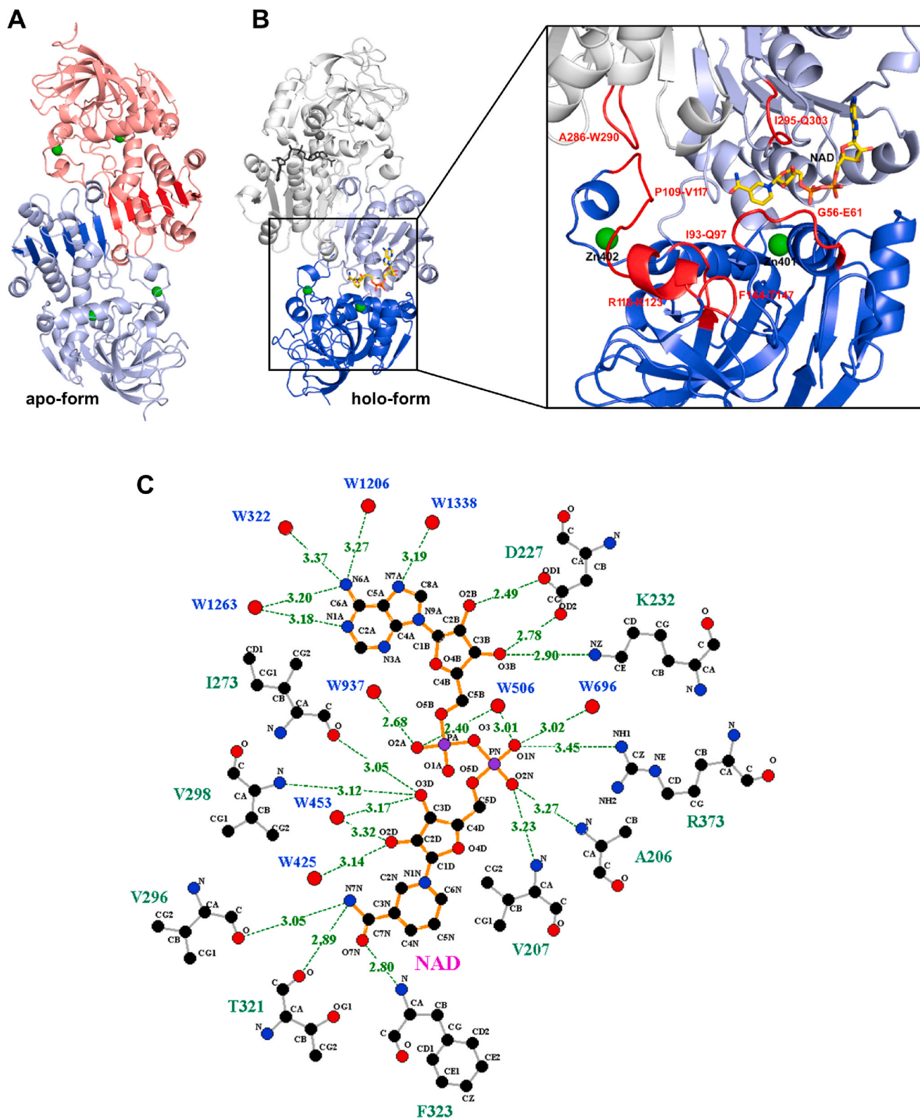
Fig. 3. Crystal structure of apo- and \text{NAD}^+ -CrGSNOR1. (A) Overall folding of dimeric apo-CrGSNOR1. The two subunits are shown in salmon and light blue and the zinc ions of each subunit as green spheres. The six \beta -strand of each subunit forming a continuous \beta -sheet at the dimer interface are highlighted in red and blue. (B) Overall folding of dimeric \text{NAD}^+ -CrGSNOR1. \text{NAD}^+ shown in sticks occupies the cofactor-binding domain (in light blue; residues 178–326) characterized by the typical Rossman fold. The larger catalytic domain (in blue; residues 1–177 and 327–377) comprises the metal ion sites. The active site of CrGSNOR1 (zoom) is located between the catalytic and cofactor-binding domains and is formed by the loops and the \alpha -helix highlighted in red. (C) Hydrogen bond and salt-bridge interactions (up to 3.5 Å) of \text{NAD}^+ with protein residues and water molecules. (For interpretation of the references to colour in this figure legend, the reader is referred to the Web version of this article.)
