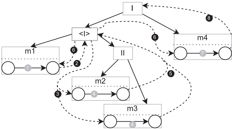
Fig. 2. Visit of a compositional simulation tree for (m_1 \langle | \rangle (m_2 \parallel m_3)) \mid m_4 .
