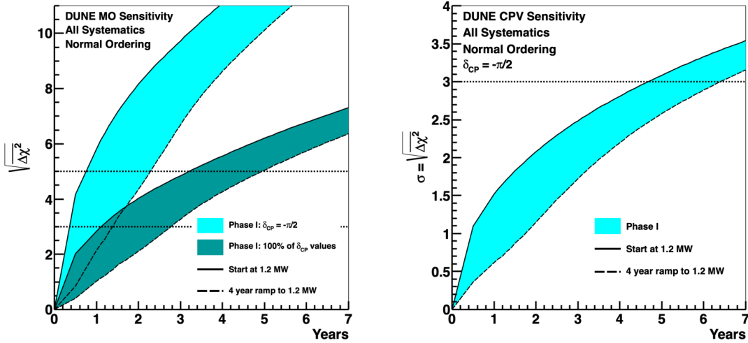
FIG. 5. Sensitivity to the neutrino mass ordering (left) and CP violation for \delta_{CP} = -\pi/2 (right) in Phase I. The cyan bands show the sensitivity if \delta_{CP} = -\pi/2 and the green band in the left plot shows the sensitivity for 100% of \delta_{CP} values. The width of the bands shows the impact of potential beam power ramp up; the solid upper curve is the sensitivity if data collection begins with 1.2 MW beam power and the lower dashed curve shows a conservative beam ramp scenario where the full power is achieved after 4 years.
