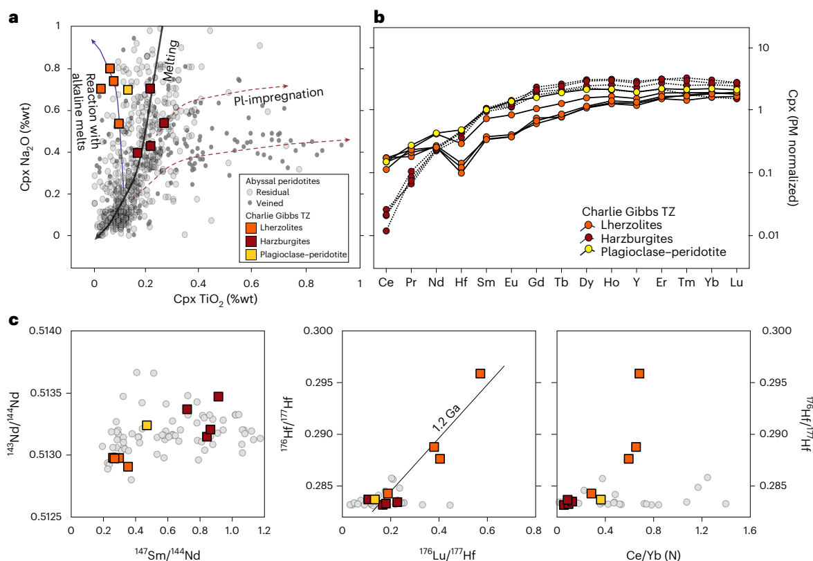
Fig. 2 | Major, trace elements and Nd–Hf isotopes of Charlie Gibbs peridotites.
