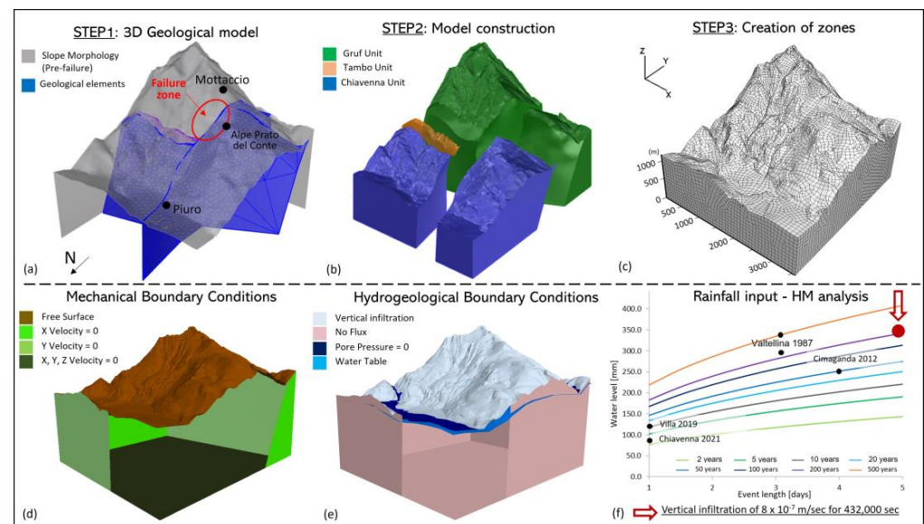
Figure 4. (a) 3D geological model built starting from the geological–structural features of the slope presented in Figure 1d; (b) FLAC3D model building; (c) Discretization into a finite-difference grid by the definition of hexahedral zones; (d) Boundary conditions of the mechanical model; (e) Boundary conditions of the hydrogeological model for the hydro-mechanical analysis; (f) Rainfall input of hydro-mechanical analysis. Identification of input values by evaluating rainfall scenarios in the study area.
