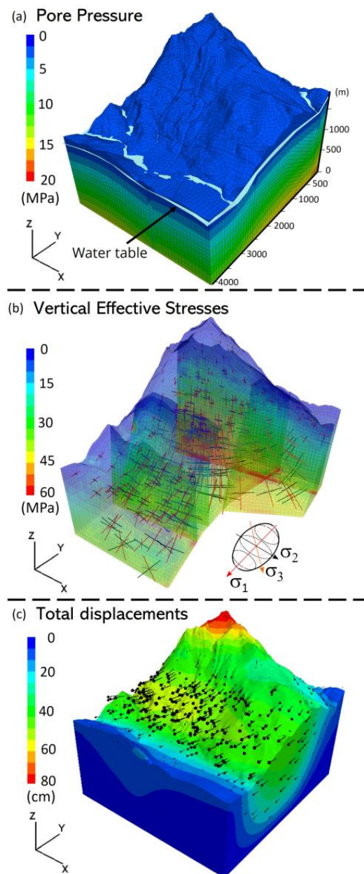
Figure 5. Pore pressures (a), effective stresses (b), and total displacements (c) simulated along the modelled slope at initialization phase.
