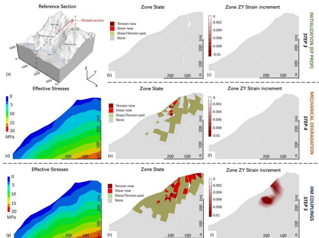
Figure 6. (a) Location of the 2D section showing effective stresses (d,g), zone state (b,e,h), and ZY strain increment (c,f,i) simulated for different steps of the analysis.
