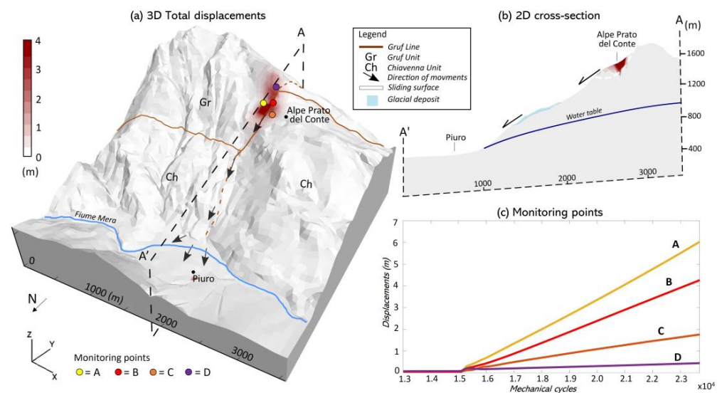
Figure 7. (a) 3D total displacements simulated at the end of the HM coupled analysis. (b) 2D total displacements along a N-S cross-section crossing the failure area. (c) Graph of measured displacements at monitoring points (Figure 6a) with mechanical cycles (defined as the number of timesteps performed).
