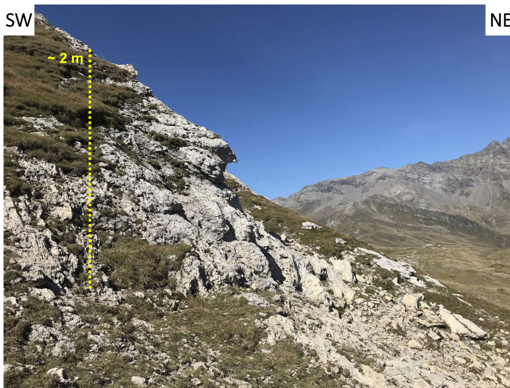
Fig. 41 - Carnieule outcrop in the upper part of Valle dei Buoi, along the path to Monte Tignoso.
