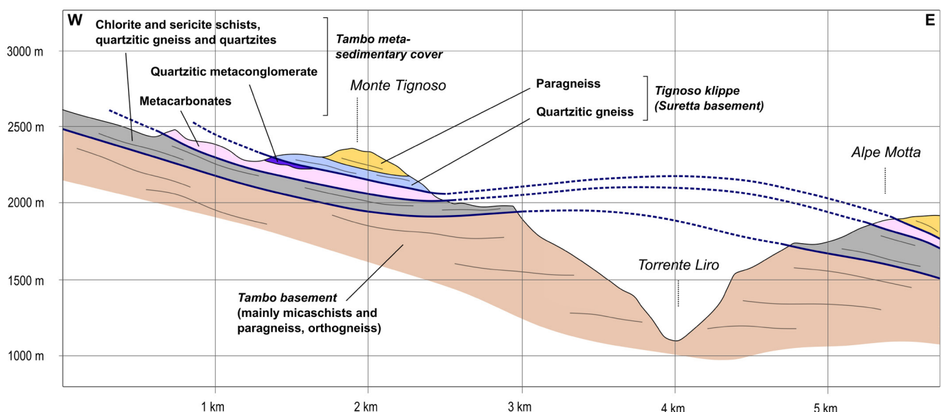
Fig. 6 - Geological cross-section of Val San Giacomo through the Monte Tignoso area.
