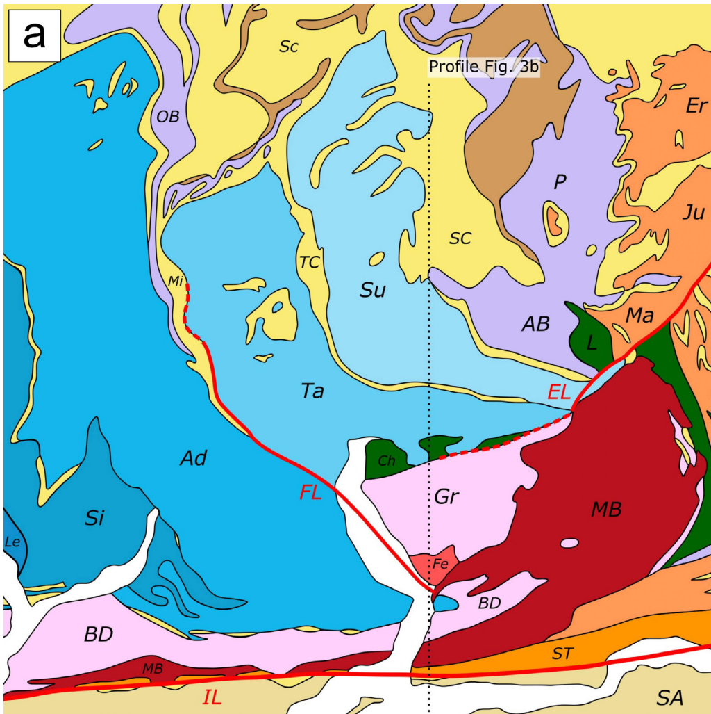
Fig. 3 - a) Simplified tectonic map of the Central Alps (redrawn after Spicher, 1980). Abbreviations: AB = Avers nappe; Ad = Adula nappe; BD = Bellinzona-Dascio Zone; Ch = Chiavenna Unit; EL = Engadine Line; Er = Err nappe; Fe = Novate Granite; FL = Forcola Line; Gr = Gruf Complex; IL = Insubric Line; Ju = Julier nappe; L = Lizun Ophiolite; Le = Leventina nappe; Ma = Margna nappe; MB = Bergell Pluton; Mi = Misox Zone; SC = Suretta meta-sedimentary cover; P = Platta nappe; SA = Central Alps Southalpine; Sc = Schams nappes; Si = Simano nappe; TC = Tambo meta-sedimentary cover; Su = Suretta nappe.; b) synthetic tectonic cross-section of the Central Alps along Valchiavenna and Val di Lei (redrawn after Schmid et al., 1990).
