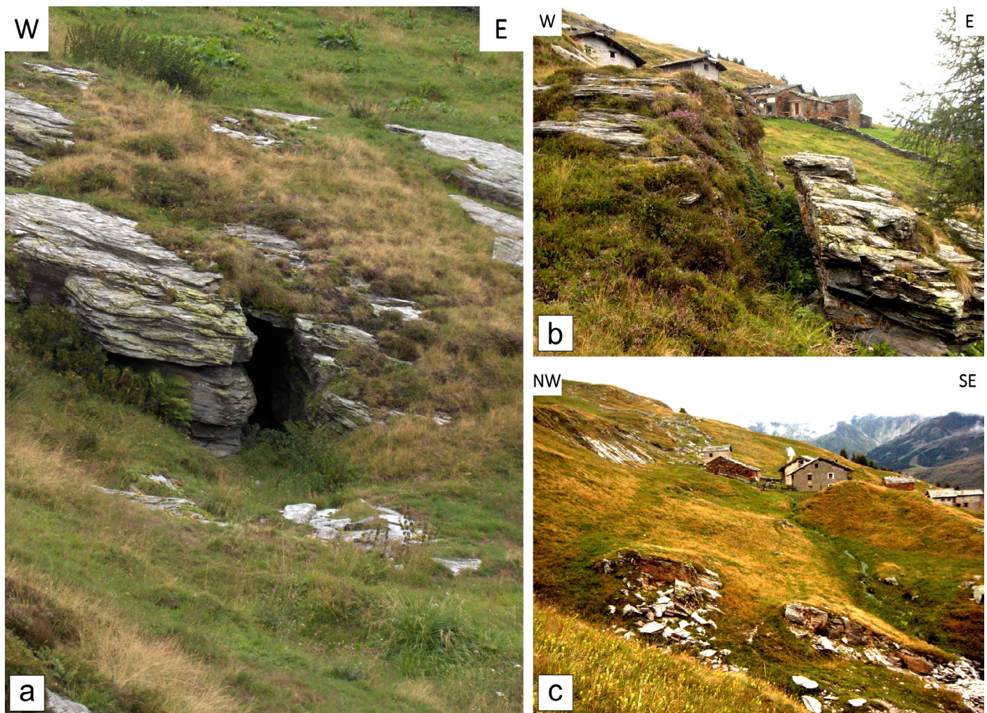
Fig. 11 - a) and b) Meter-sized open fractures on the slope south of Alpe Toiana; c) trenches at Alpe Toiana.
