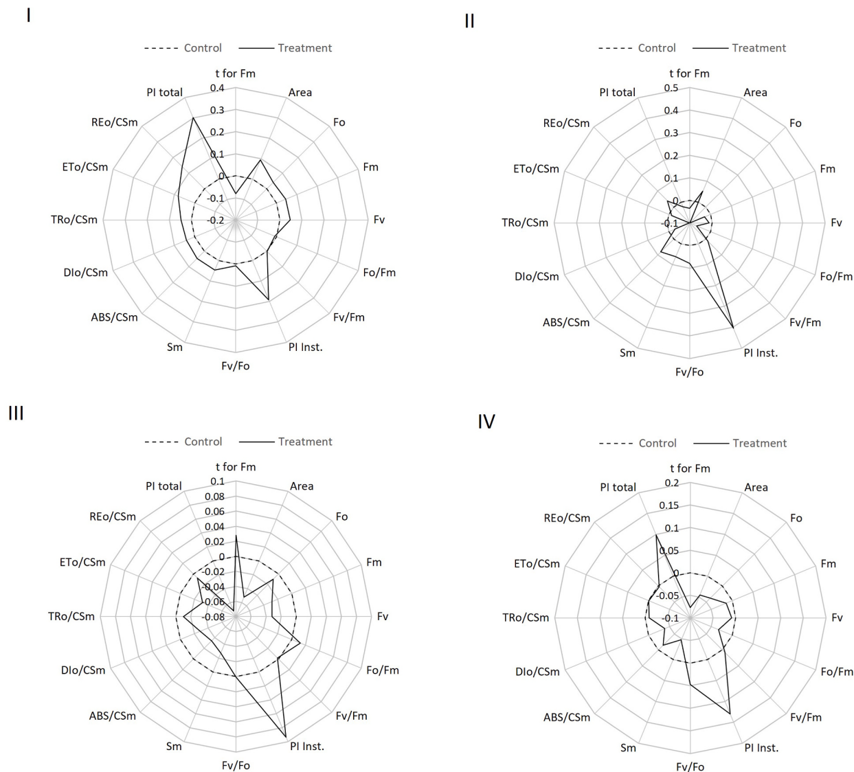
Fig. 3. Chlorophyll a fluorescence parameters measured in vivo in red (Codex) lettuce leaves. Measurements were taken 2 days after the first (I), the second (II), the third (III) application, and at harvest (IV). Values are means \pm SE ( n = 6 ). (F_t - F_c)/F_c was used to normalize the data. In the formula, “ F_t ” and “ F_c ” represent the values of treated plants and control plants treated with water, respectively. Values of “ F_c ” plants were normalized to 0 (control plants treated with water, dotted line circle = 0).
