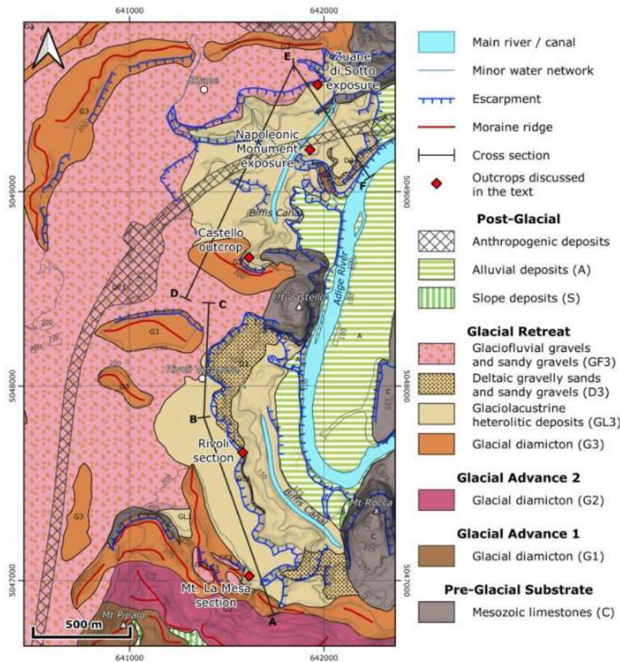
Fig. 3 - Quaternary geological sketch map of the AMA innermost moraine ridge. The glacial units are summarized into three groups, based on morphostratigraphic criteria: Glacial Advance 1, Glacial Advance 2, Glacial Retreat. Furthermore, we reported also Pre-Glacial Substrate (Mesozoic limestones, Venzo et al., 1969; Accorsi et al., 1990) and Post-Glacial deposits. The outcrops and stratigraphic sections described in this paper are highlighted. Smaller kame terraces are highlighted on the northern flank of Mt La Mesa by glaciofluvial deposits (GF3). Cross sections are represented in Fig. 5.
