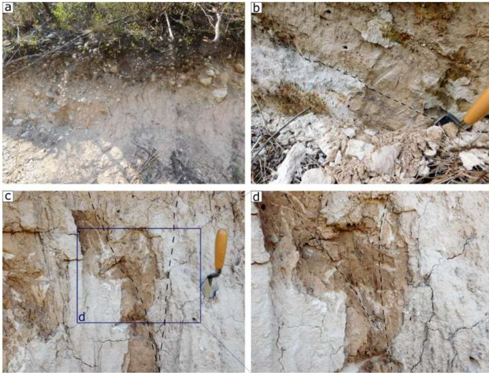
Fig. 8 - Castello outcrop, northern sector. (a) Global vision of the outcrop. Gravel scours, characterized by clast-supported massive pebbly gravel (deltaic facies association D) are highlighted by an erosional surface above glaciolacustrine facies association GL. (b) Particular showing normally graded sand (glaciolacustrine facies association GL); the dotted line highlights the inclined lamination. (c) Ice-wedge cast within mud-prone deposit (glaciolacustrine facies association GL); the dotted line evidences the cast. (d) Particular from Fig. 8c, showing vertical and high-angle inclined lamination highlighted by dotted lines.
