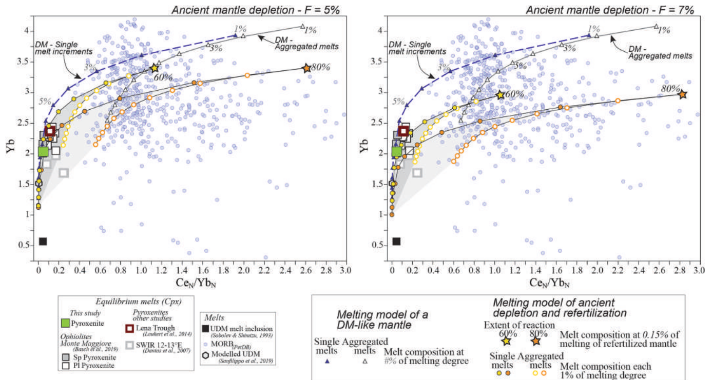
Fig. 8. Diagrams showing Ce_N/Yb_N ( N = Chondrite-normalized values) vs Yb compositions of melts calculated in equilibrium with clinopyroxenes in pyroxenite veins from modern mid-ocean ridges (Doldrums FZ, this study; Lena Trough [average composition], Laukert et al., 2014; 12°-13° E SWIR, Dantas et al., 2007) and ophiolitic analogues (Monte Maggiore Ophiolite, Corsica, Basch et al., 2019). For comparison we also show the compositions of MORBs (compiled from PetDB, www.earthchem.org/petdb ) and of the ultra-depleted melts documented in an olivine-hosted inclusion (Sobolev and Shimizu, 1993) and modelled by numerical melting models (Sanfilippo et al., 2019). Also shown are the expected Ce_N/Yb_N vs Yb evolution lines for melts produced by partial melting in the spinel stability field of a depleted mantle (DM) source (lines with triangles) and of ancient, residual mantle sources after 5% (A) and 7% (B) ancient melting that were modified by increasing extents of melt-rock reactions (60%: yellow star and dots, 80%: orange star and dots). A dynamic melting model was used assuming melting within the spinel-stability field exclusively and a fixed residual porosity of 1%; partition coefficients are from Salters and Stracke (2004). The DM source is from Workman and Hart, 2005. The starting composition of ancient, purely residual and refertilized mantle is taken from the numerical models performed by Sani et al. (2023); see the text and Fig. 7 for further details. Solid dots and triangles indicate composition of single melt increments, whereas the empty dots and triangles indicate the compositions of aggregated melts. The stars show melts produced after 0.15% melting of the selected ancient, refractory and refertilized mantle sources. (For interpretation of the references to colour in this figure legend, the reader is referred to the web version of this article.)
