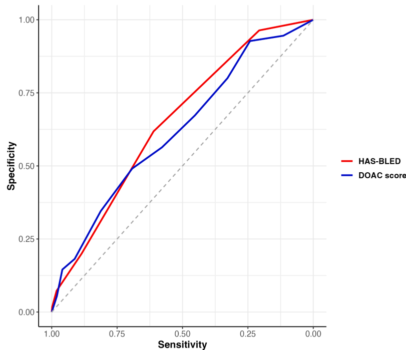
Fig. 2. Area under the curve for prediction of Major Bleeding for HAS-BLED and DOAC score AUC [95 % CI] HAS-BLED score: 0.65 [0.55-0.70]; AUC [95 % CI] DOAC score: 0.62 [0.59-0.71]. DeLong's test for difference: Z = -0.97 , p -value = 0.332 AUC, area under the curve; CI, confidence interval.
