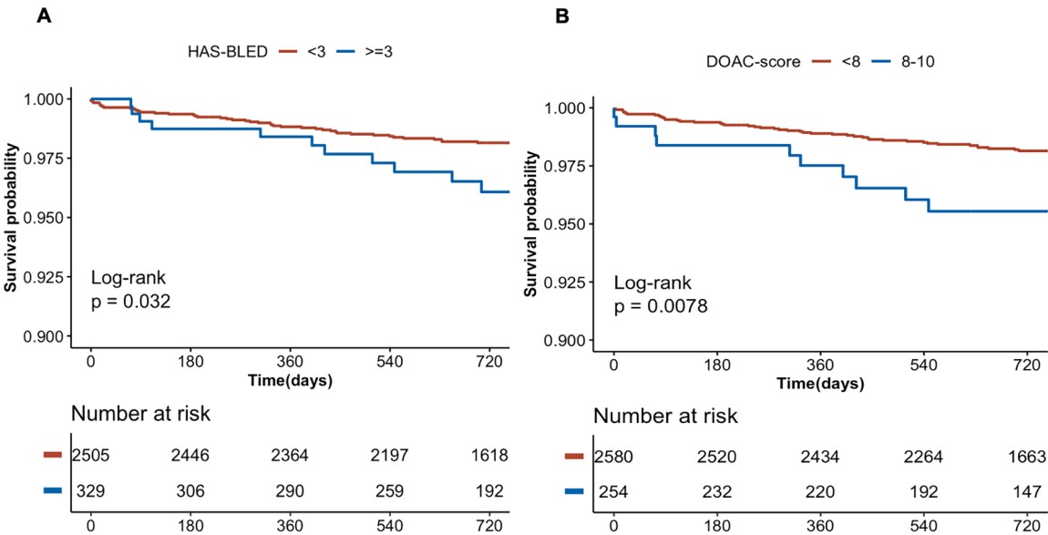
Fig. 1. Kaplan-Meier curves for Major Bleeding. Panel A shows the cumulative incidence of major bleeding events categorized by HAS-BLED. Panel B shows the cumulative incidence of major bleeding events categorized by DOAC score.
