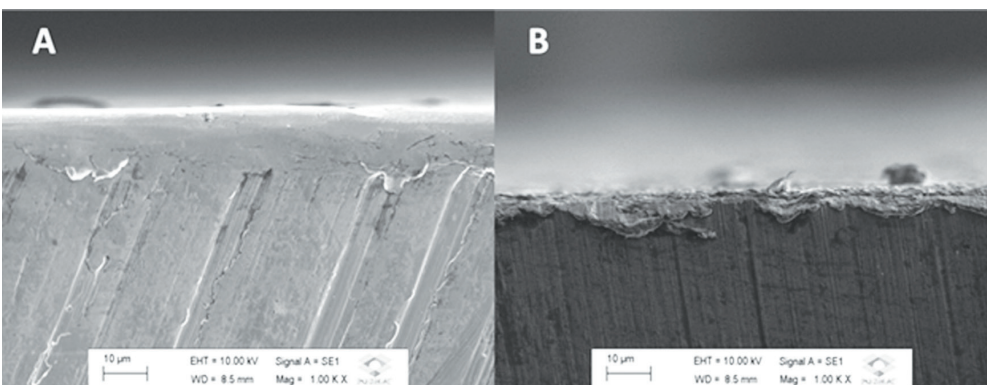
FIG. 4 SEM cross section of the disks of the MS (A) and AFS (B) groups (1000x).
