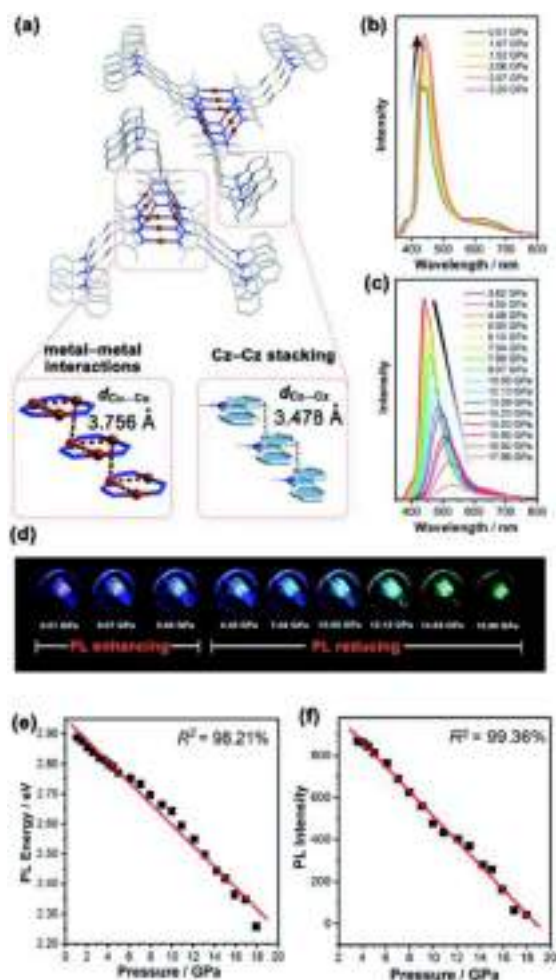
Fig. 40 (a) The crystal packing of 3.35b at 298 K, showing the infinite chain stacking model of Cz and Cu 3 . The emission spectra of 3.35b in a range of external pressures from (b) 0.01–3.20 GPa and (c) 3.62–17.96 GPa at an excitation wavelength of 355 nm. (d) Photoluminescence photographs of the 3.35b crystal under compression up to 15.90 GPa. Linear fitting of the external pressure and (e) photoluminescence energy and (f) intensity of 3.35b . Reprinted with permission from ref. 234 under the terms of the Creative Commons license. Copyright 2021, The Royal Society of Chemistry.
