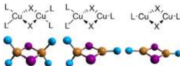
Scheme 10 Structure of complexes with \{\text{Cu}_2\text{X}_2\} cores: left – [(\text{Cu}_2\text{X}_2)\text{L}_4] , centre – [(\text{Cu}_2\text{X}_2)\text{L}_3] and right – [(\text{Cu}_2\text{X}_2)\text{L}_2] .
