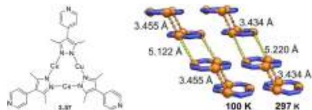
Fig. 44 Left: chemical structure of 3.37. Right: the face-to-face stacking diagrams shown by Cu_3N_6 rings and intermolecular Cu\cdots Cu distances at 100 K and 297 K. Colour code: orange, Cu; blue, N. Adapted with permission from ref. 242. Copyright 2023, The Royal Society of Chemistry.
