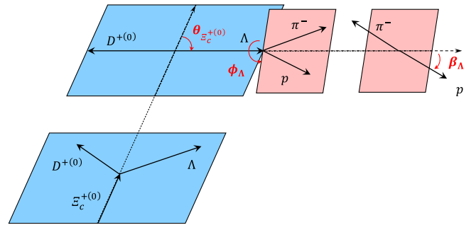
FIG. 5. Definition of the three angular variables \cos\theta_{\Xi_c} , \phi_{\Lambda} , and \cos\beta_{\Lambda} . The variable \theta_{\Xi_c^{+(0)}} is the angle between the \Lambda momentum and the momentum of the pion from the \Xi_b^{0(-)} decay, in the rest frame of the D^{+(0)}\Lambda system (denoted as \Xi_c^{+(0)} ), and is referred to as the \Xi_c^{+(0)} helicity angle. The \Lambda helicity angle \beta_{\Lambda} is defined by the momentum of the proton and that of the D^{+(0)} meson in the \Lambda rest frame. The variable \phi_{\Lambda} is the angle between the \Xi_c^{+(0)} \rightarrow D^{+(0)}\Lambda and \Lambda \rightarrow p\pi^- decay planes.
