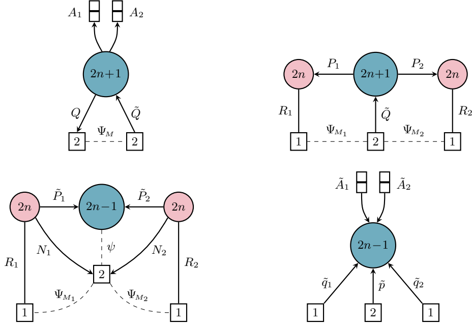
Figure 8. Deconfinement steps of SU(2n+1) with two antisymmetrics, two fundamentals and two antifundamentals.
