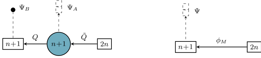
Figure 14. In this figure we represent the quivers associated to the duality between SU(n+1) with an antisymmetric Fermi and the LG model. Dashed lines are for Fermi fields while continuous lines are for chiral multiplets. The dots refer to the singlets.
