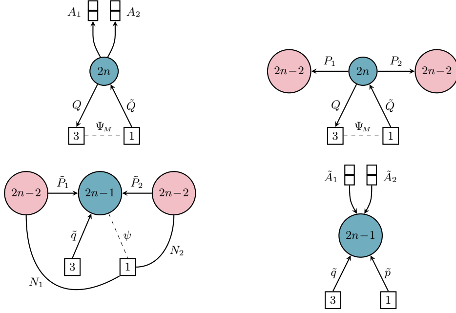
Figure 5. Deconfinement steps of SU(2n) with two antisymmetrics, three fundamentals and one anti-fundamental.
