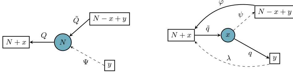
Figure 2. Quiver diagrams of the electric theory (left) and the magnetic theory (right).
