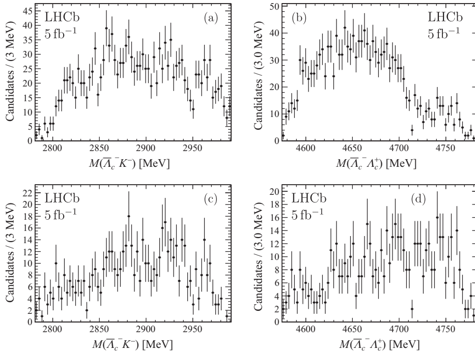
FIG. 4. Mass spectrum of (a), (c) \bar{\Lambda}_c^- K^- and (b), (d) \Lambda_c^+ \bar{\Lambda}_c^- pairs from (a), (b) all the B^- \rightarrow \Lambda_c^+ \bar{\Lambda}_c^- K^- candidates and (c), (d) after vetoing candidates with 2900 < M(\Lambda_c^+ K^-) < 2970 MeV.
