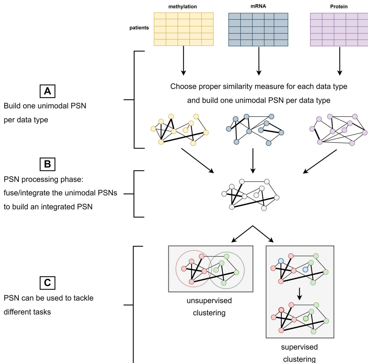
Figure 2. High-level representation of PSN-fusion methods. (A) Given a set of matrices, each representing the patients vectors acquired from one source, proper similarity measures or kernel functions are used to build a set of unimodal PSNs (one PSN per data source or data type); (B) all the PSNs are then fused through either MKL methods, SNF methods or other PSN-fusion approaches; (C) the integrated PSN is processed either by unsupervised clustering algorithms for solving, e.g. patients' subtype prediction tasks, or by supervised classifier models for, e.g. patients' outcome prediction.
