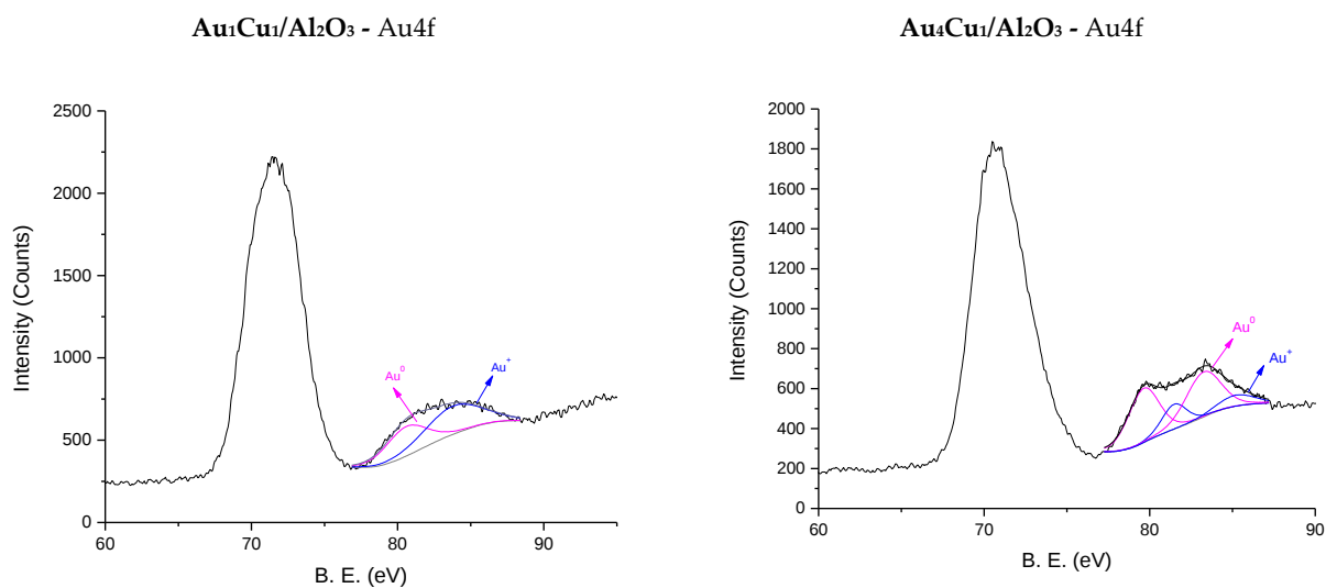
Figure S4. Au 4f deconvolution for A) Au 1 Cu 1 B) Au 4 Cu 1 Al 2 O 3 -supported catalysts.
