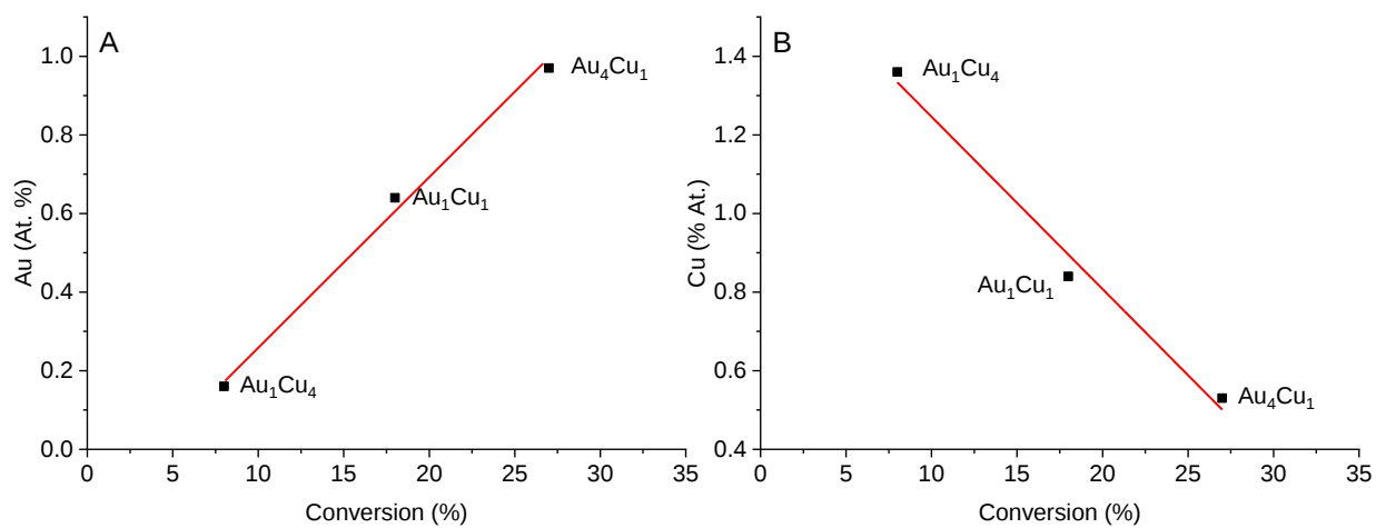
Figure S5. Influence of A) gold and B) copper surface exposure on the conversion of VA after 1 h for Al 2 O 3 supported catalysts.
