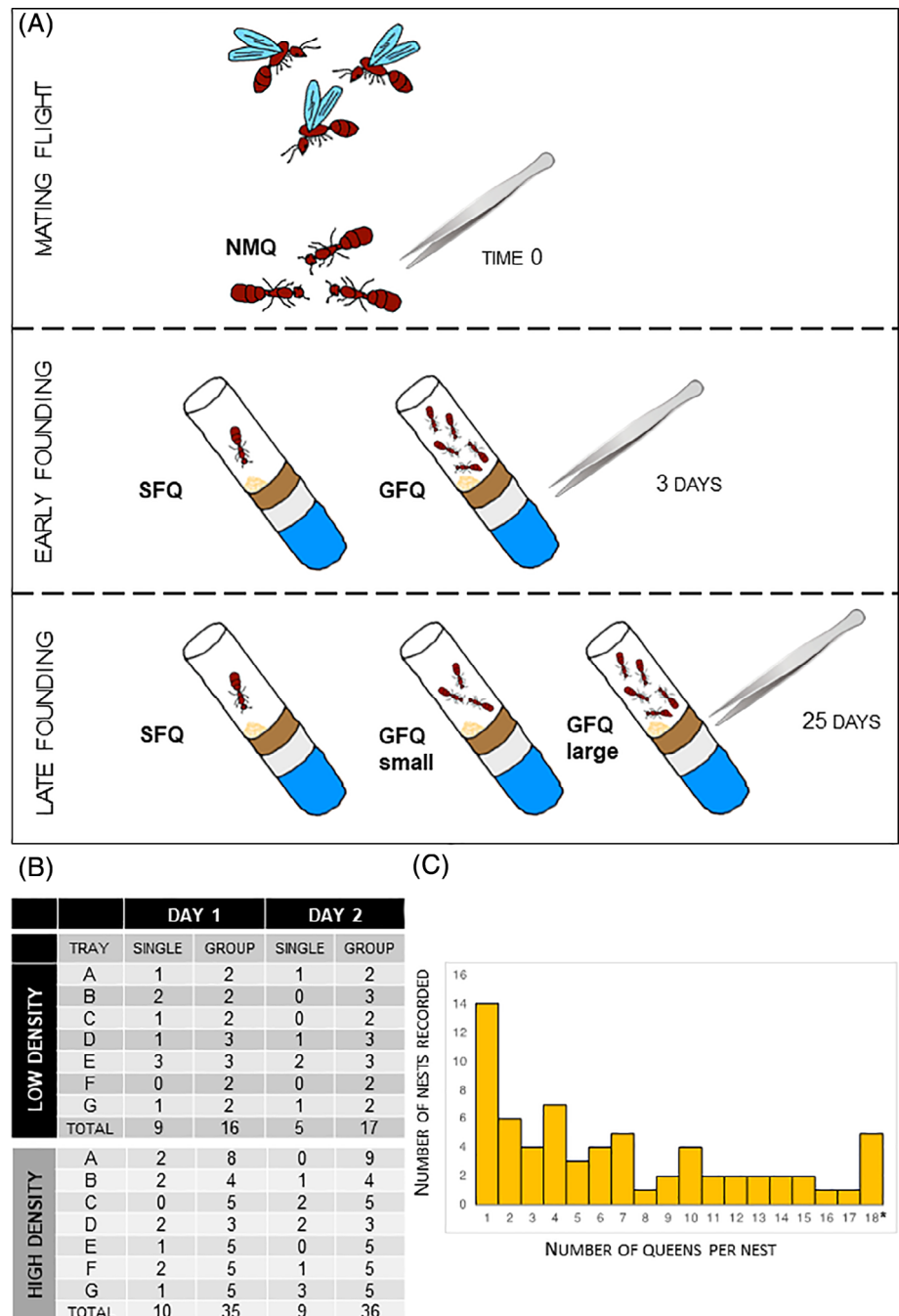
FIGURE 1 Experimental setup and sample collections. (A) Queens were sampled after a mating flight and reared in artificial nesting chambers in the lab. Focal queens were frozen at three key time points for RNA sequencing: 0, 3 and 25 days post-founding. (B) Numbers of individual queens and associations that were recorded during the first 2 days of the process when different availabilities of nesting sites were simulated: large trays with abundant nests (“low density” of queens) or small trays with fewer nests (“high density” of queens). (C) Proportions of individual queens and groups of different size that were observed at day 2 post-founding. Note: This category includes founding groups of 18 or more queens (maximum recorded = 30). GFQ, group-founding queens from small (2–6 queens) and large groups (8–21 queens); NMQ, newly mated queens; SFQ, single-founding queens
