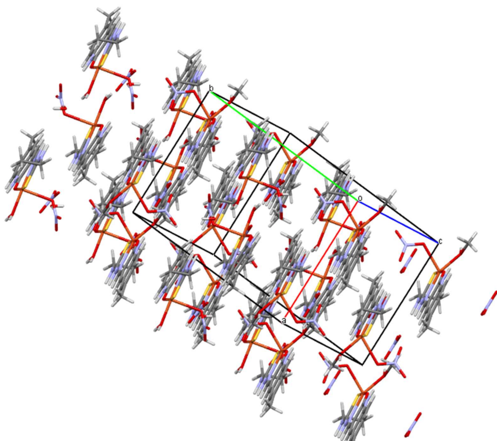
Figure S14. Molecular Packing of 3.
