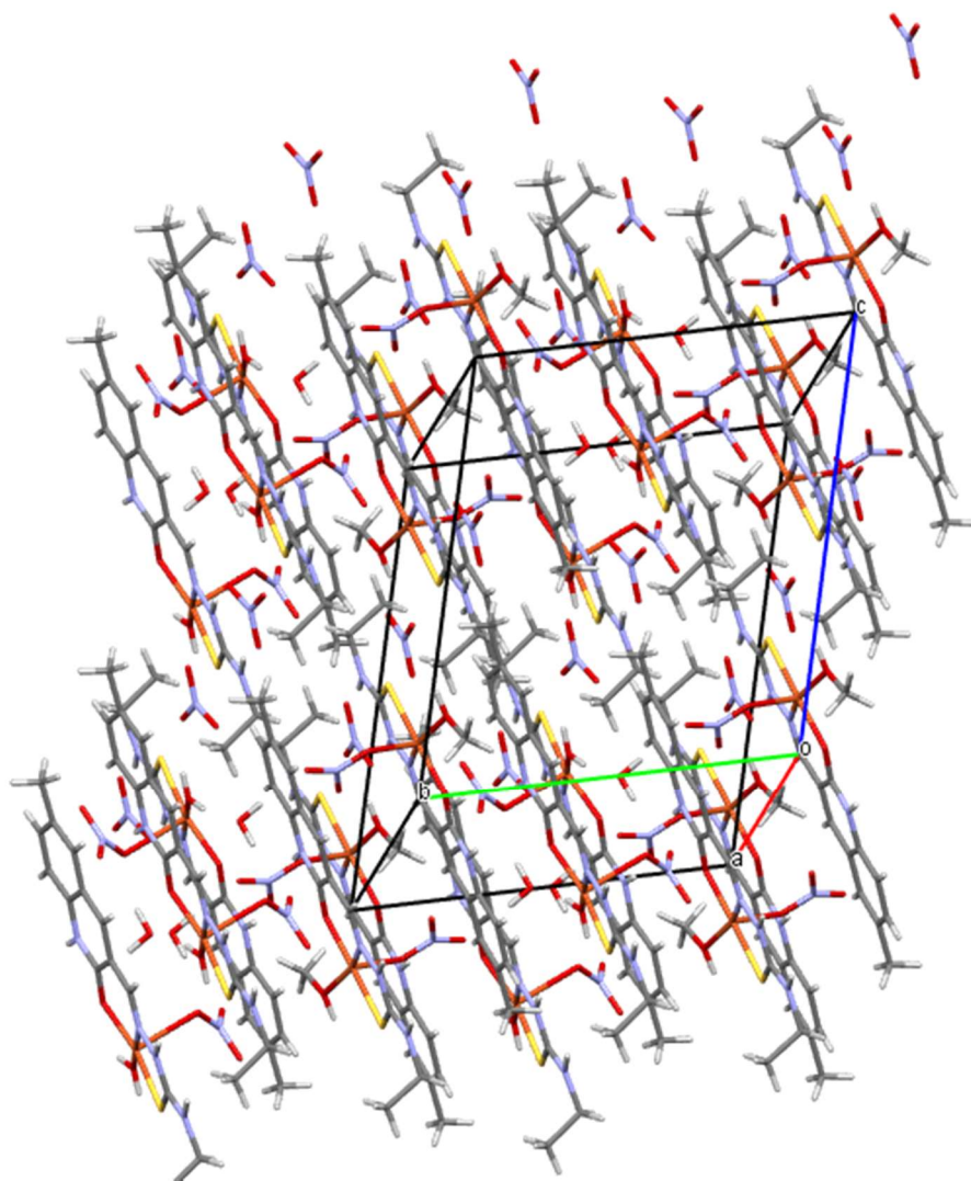
Figure S15. Molecular Packing of 3.
