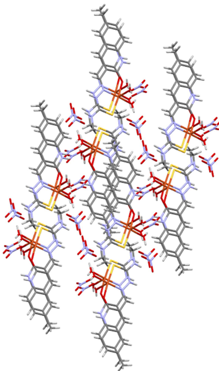
Figure S4. Packing view of 2 showing the \pi - \pi stacking between the aromatic part of the ligands.
