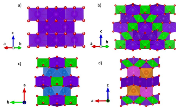
Fig. 1 Unit cell of fluorite (a) ( s.g. Fm\bar{3}m ) and pyrochlore (b) ( s.g. Fd\bar{3}m ) structure along [110]; unit cell of weberite-type structure in Cmmm space group (c) along [001] and in Pmma space group (d) along [010]. A-site cations 8-fold coordinated are in purple (Wyckoff positions 4a in a, 16d in b, 4b in c and 2b and 2c in d) and B-site cations 6-fold coordinated are in green polyhedra (Wyckoff positions 16c in b, 4a in c and 2a and 2d in d); the 7-fold coordinated site shared by both A- and B-site cations in c (blue polyhedra, Wyckoff position 8g) splits into two separate sites in d (orange and pink polyhedra, Wyckoff position 4k). Oxygen atoms are represented by red spheres.
