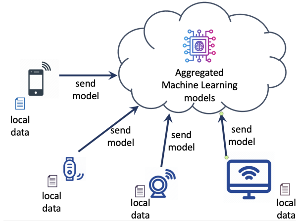
Figure 4: Federated Learning Architecture
