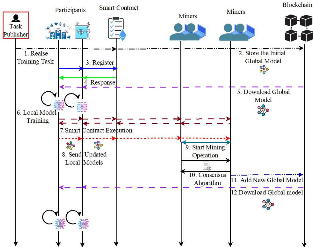
Figure 10: The high-level workflow for a single epoch Blockchain-enabled Federated Learning
