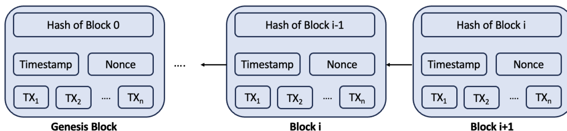
Figure 7: Example of a Blockchain
