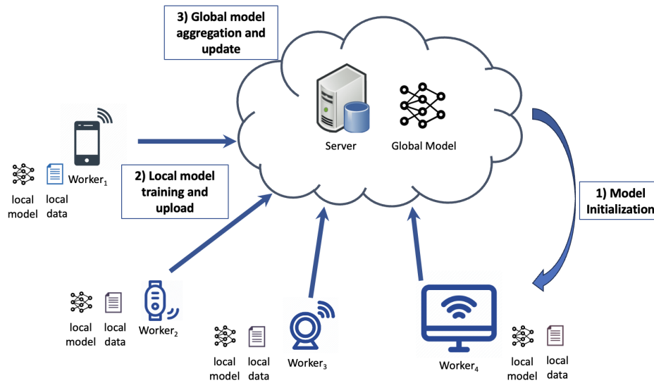
Figure 5: A schematic diagram of the Federated Learning workflow
