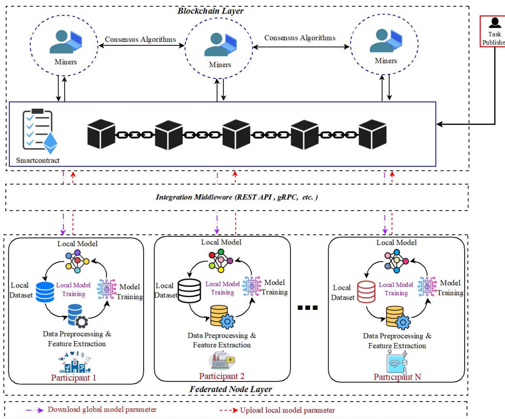
Figure 9: General architecture for the Blockchain-enabled Federated Learning.
