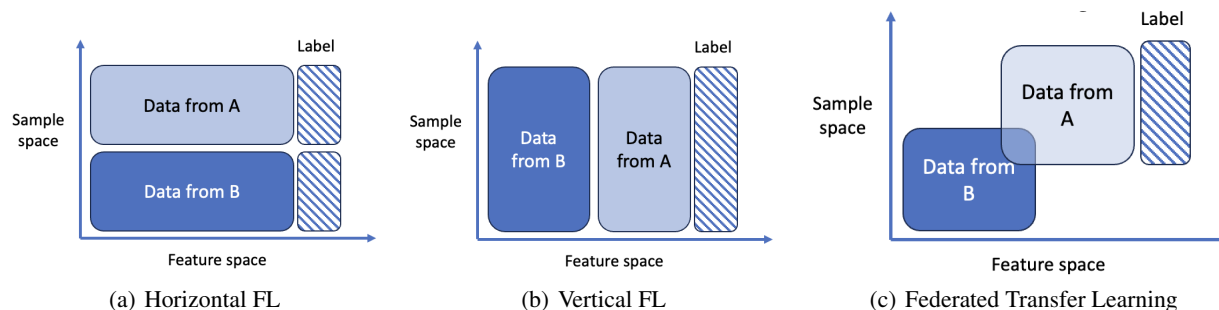
Figure 6: The three categories of FL divided for feature and sample spaces
