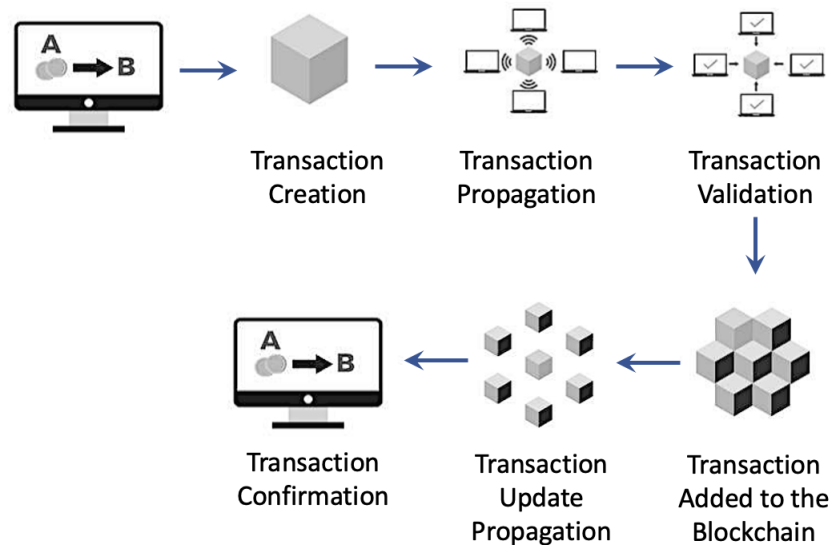
Figure 8: Transactions workflow in Blockchain
